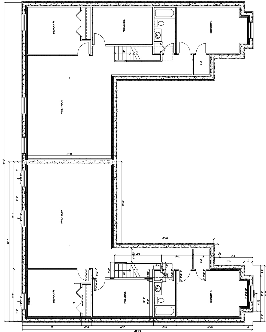
TYPE A-B BASEMENT FLOOR PLAN
