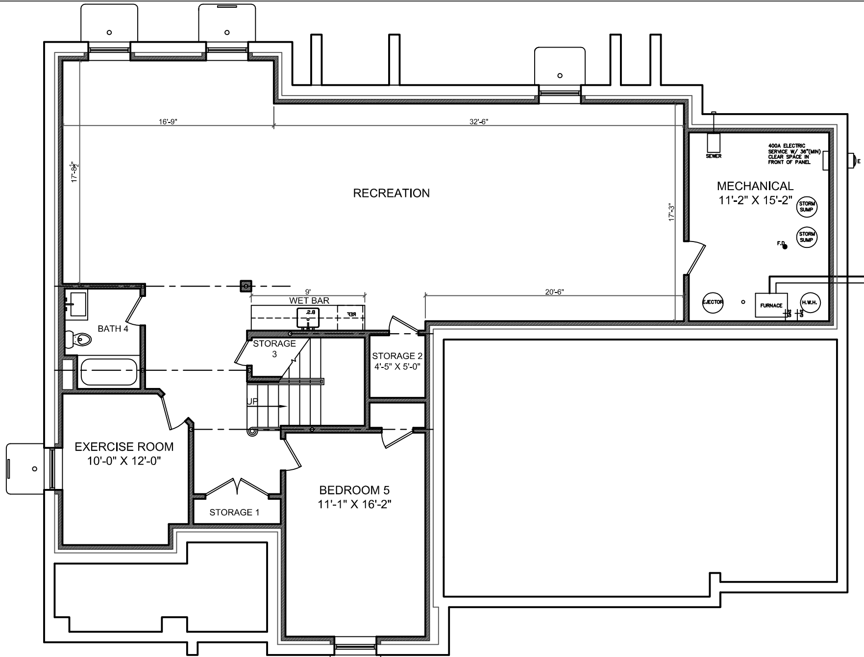
PROPOSED FINISHED BASEMENT PLAN
