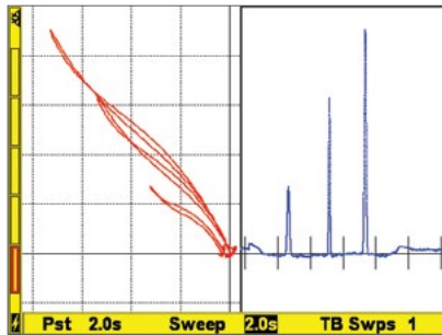
50/50 XY & Timebase
