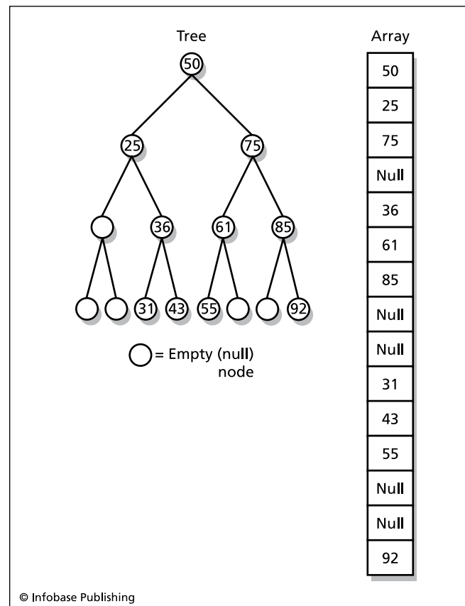
In a binary tree each node either has two branch (child) nodes or is a terminal node. Here a binary tree is shown with the equivalent representation in an array of memory locations. Notice that the numbers are stored level by level (50 in the top level, 25 and 75 in the second level, and so on.) Null would be a special value (such as -1) representing an empty node.
