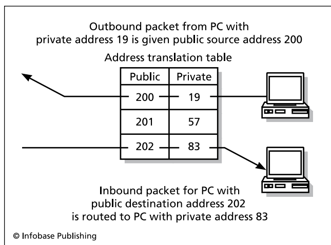
Network Address Translation (NAT) can protect computers on a local network by giving outgoing packets an arbitrary public source address in place of a computer's actual (private) address. Incoming packets addressed to that public address are then routed to the correct private address using a table.
