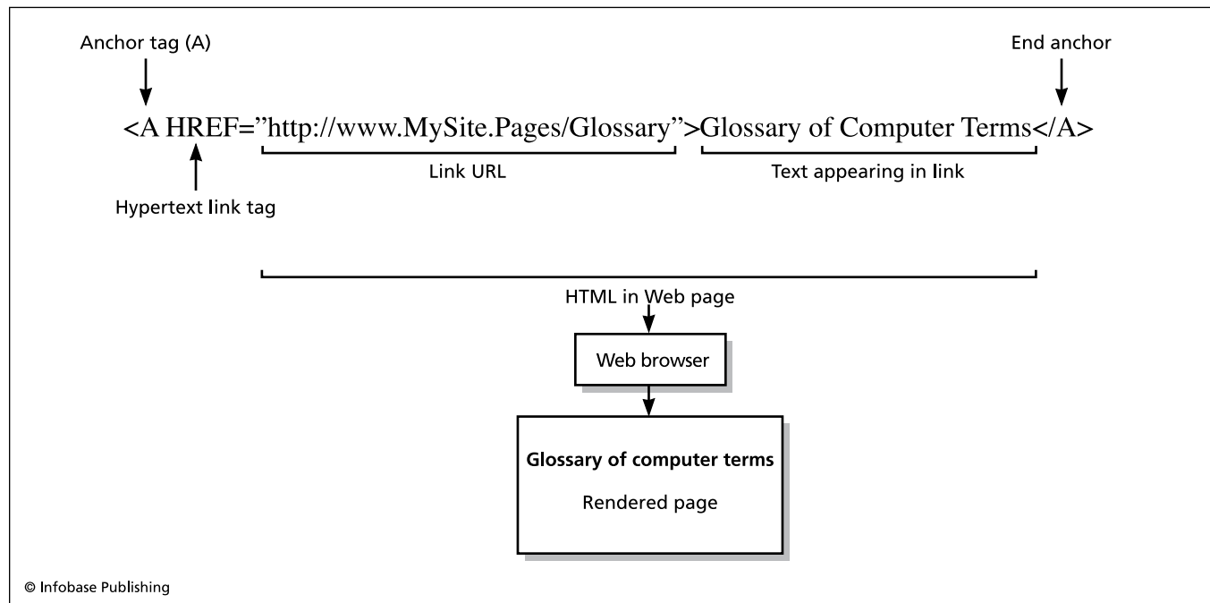
An HTML hyperlink embedded in a Web page. The anchor link gives the address (URL) of the linked page, as well as specifying the text that will appear in the link, which will be rendered by the Web browser in a special color or font.
