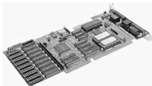
A Standard ISA bus PC expansion card. This “open architecture” allowed dozens of companies to create hundreds of add-on devices for IBM-compatible personal computers.
