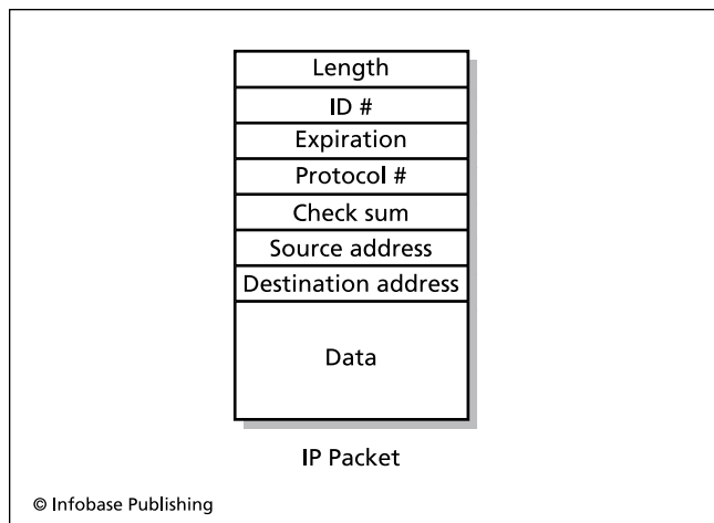
The header fields and data for an IP (Internet Protocol) packet. The packets can travel over different routes to the destination address and then be reassembled in the correct order.
