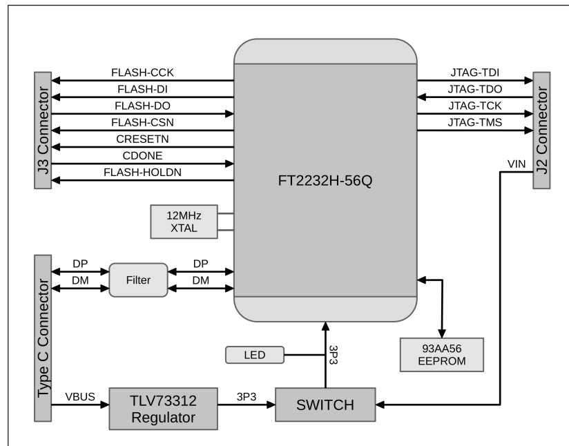
XLJTAG1 BLOCK
