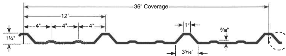
PBR Panel (Purlin Bearing Rib)
