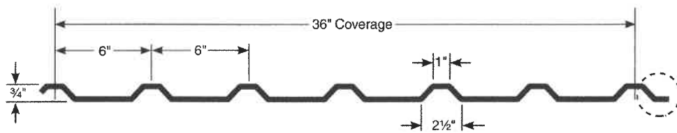
PBU Panel (Purlin Bearing Rib)
