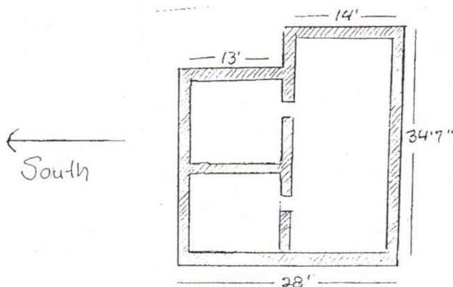
Figure 7. Original floor plan as of June 14, 1976. No insulation employed. No cooling mechanisms or overhangs. The building was kept closed during data gathering. One window on the north side. Minimal shading: large tree on the NW side of house gave partial shade on the corner late in the day.
