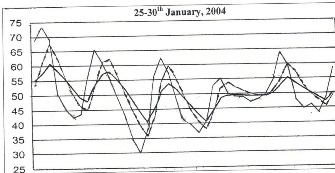
Figure 2b. Temperature data loggings for 25 to 30th of January 2004 during a cold period. Heavy black line - adobe; dashed line - cinderblock; light line - ambient temperature. Note that with respect to temperature extremes, for any given time, that the cinderblock records temperatures higher and lower than the adobe. Fluctuation of temper-
