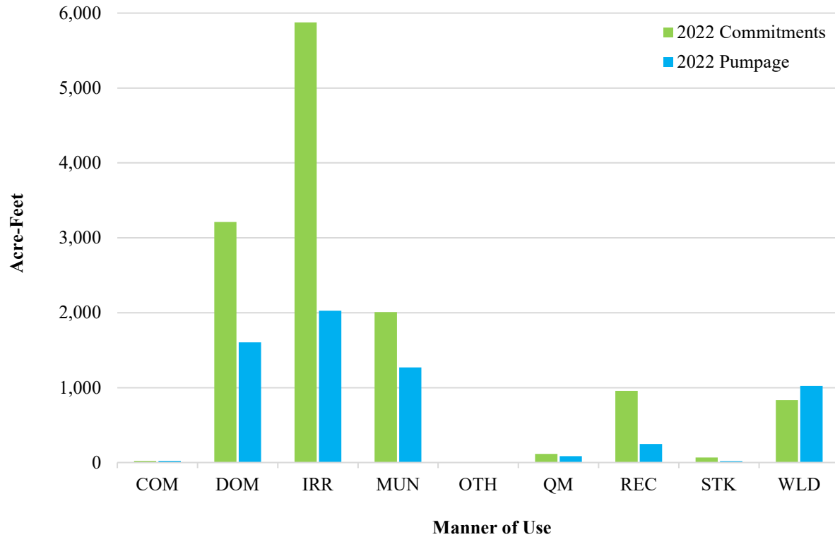
Figure 5. Comparison between 2022 groundwater commitments and estimated pumpage. Certain WLD and IRR permits in Washoe Valley share a total combined duty that is accounted for under IRR. This attribution of commitments results in WLD pumpage that exceeds WLD commitments, though over-pumping may not have occurred.
