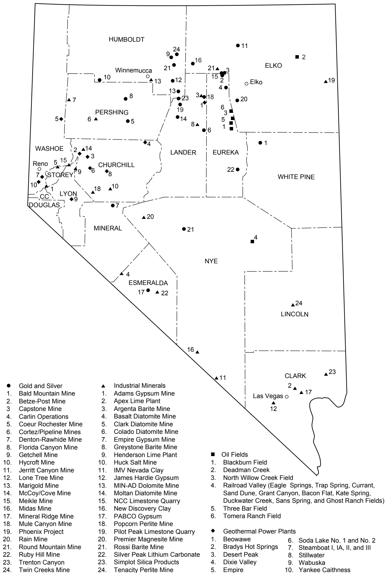
Figure 8. Major Mines, oil fields, and geothermal plants in Nevada, 2002.
