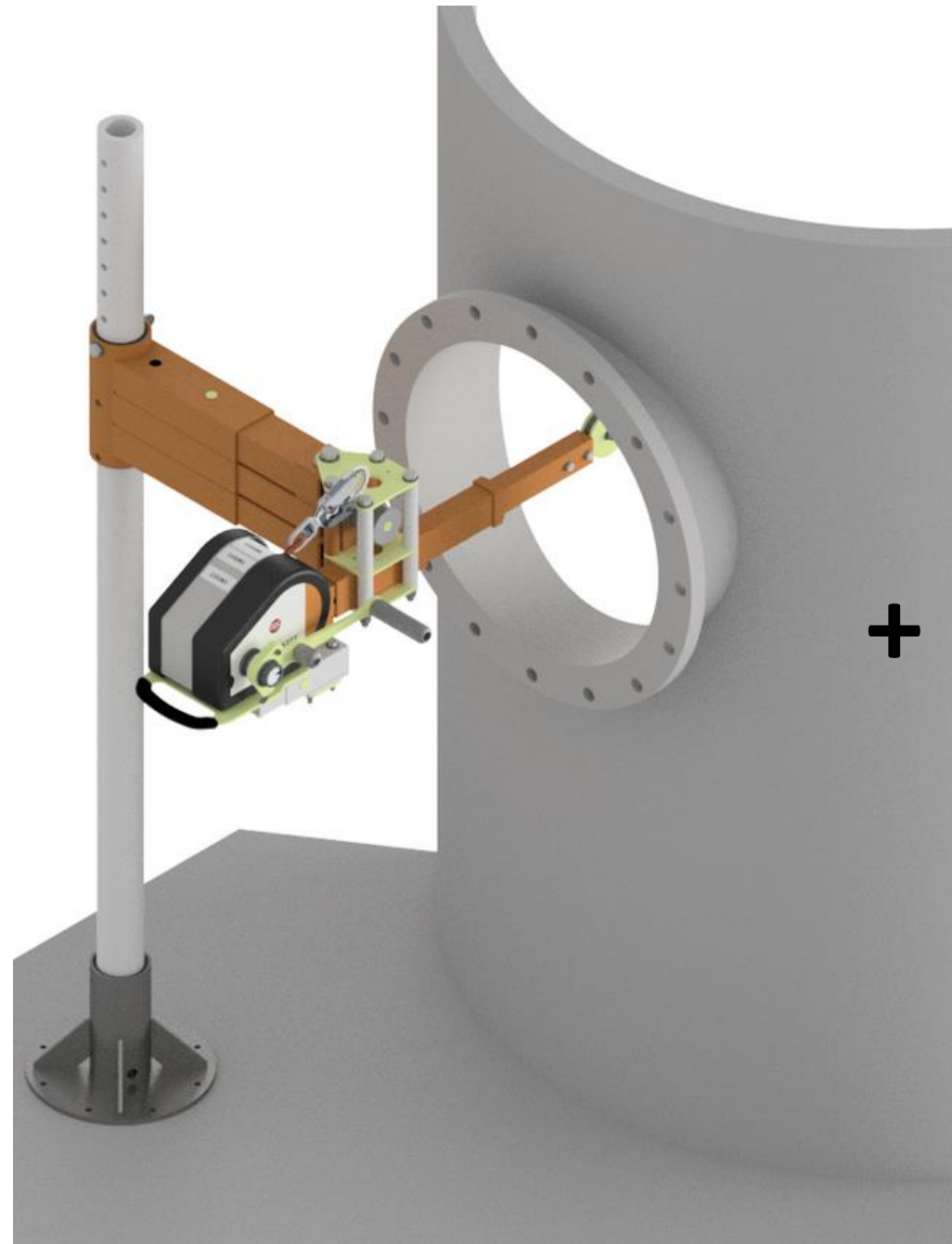
Flush Mount (Existing Concrete)
