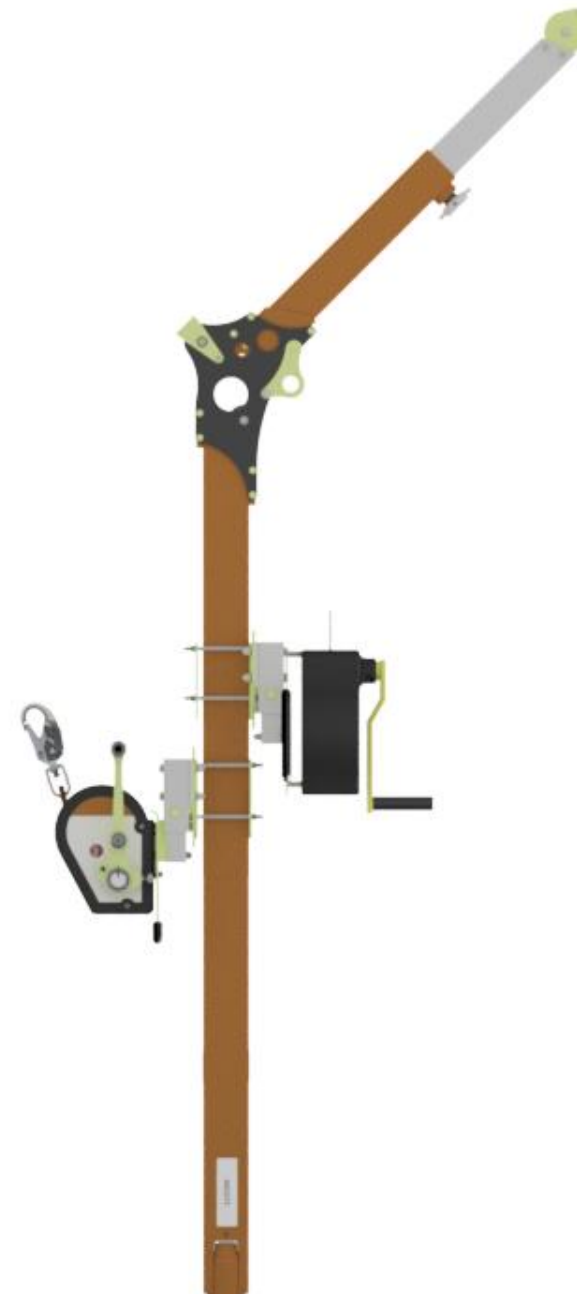
Winch and SRL-R (Require 2x60141 & 60176)
