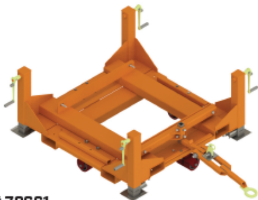
PT# 70661 Transport base for finished floor (Indoor Push/Pull)
