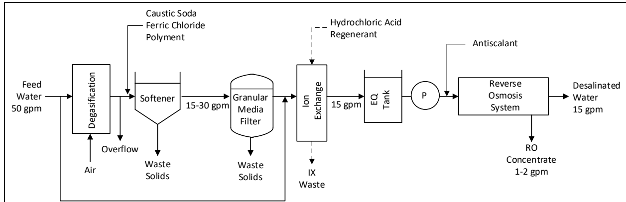
Figure 32. Process flow diagram of the desalination treatment system used for the Sandoval County Desalination Pilot Project (adapted from Universal Asset Management et al., 2011, Appendix Q).
