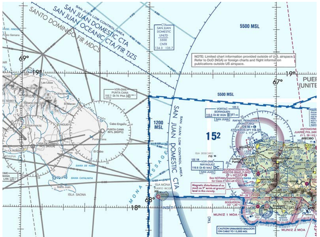
Example from Caribbean 2 VFR Aeronautical Chart
