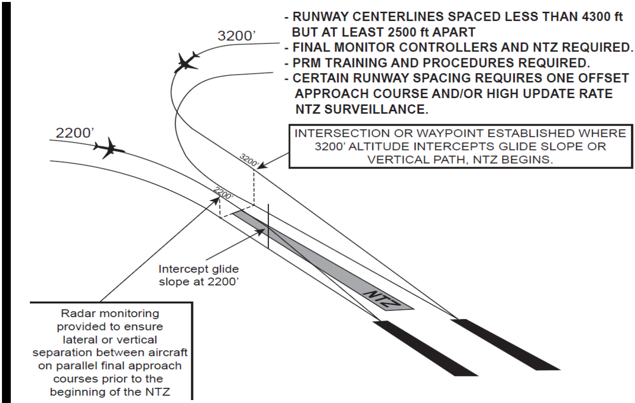
FIG 5-4-23 PRM Approaches Simultaneous Close Parallel
