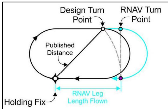
FIG 5-3-8 RNAV Lateral Guidance and Holding – No Wind
