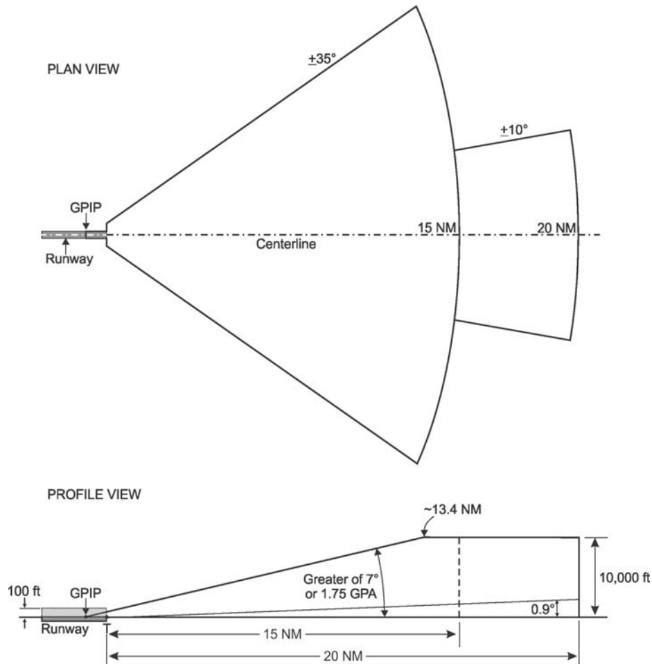
FIG 1-1-8 GLS Standard Approach Service Volume
