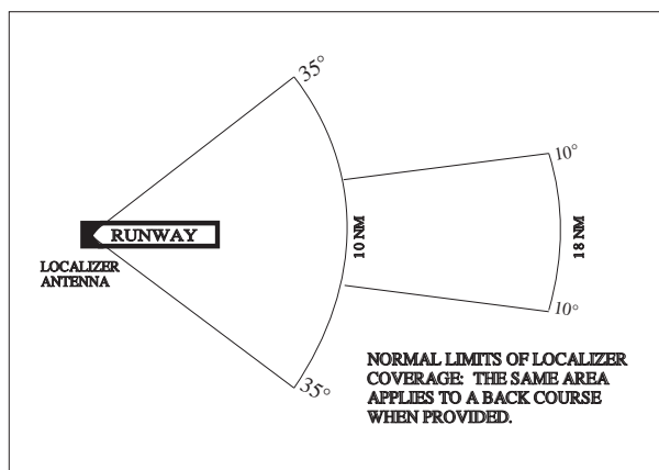
FIG 1-1-6 Limits of Localizer Coverage
