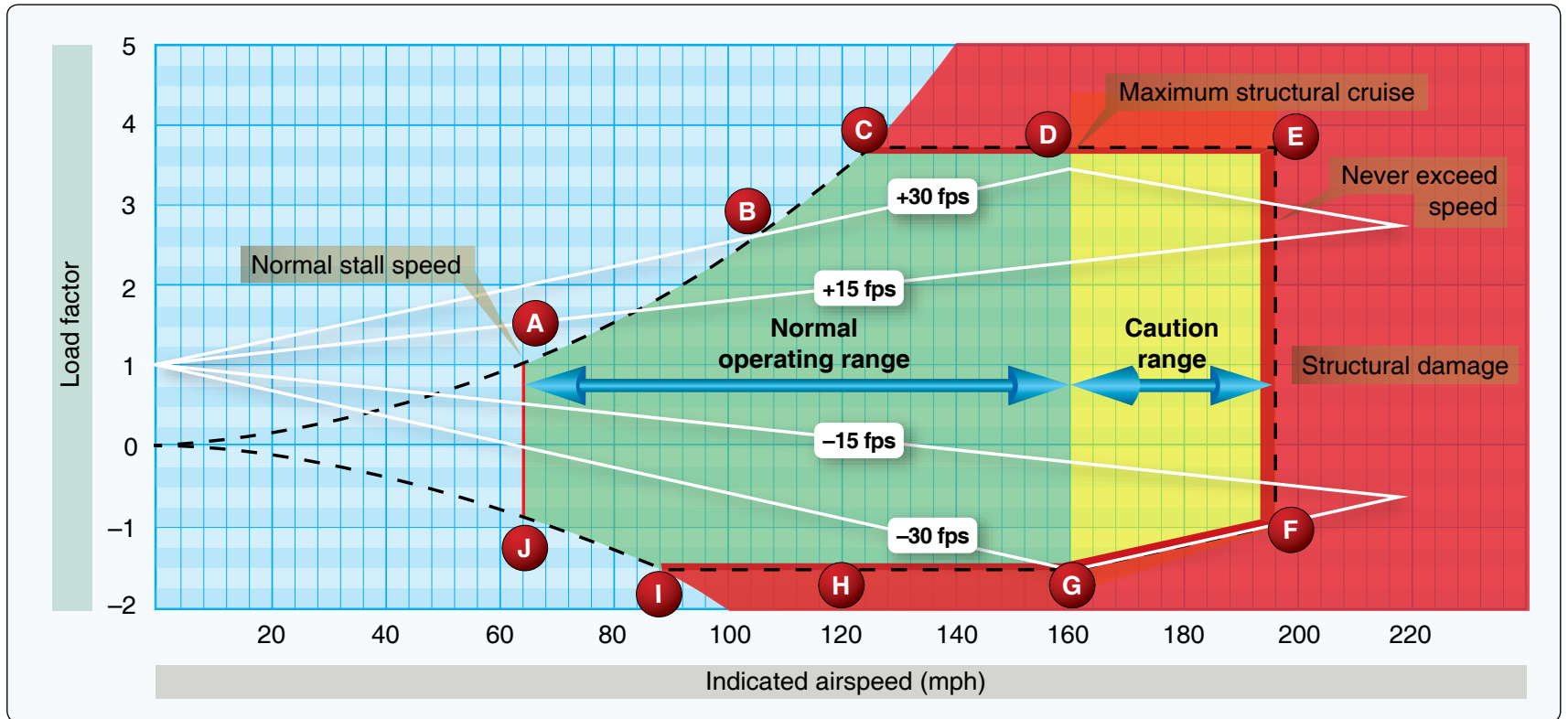
Figure 72. Velocity vs. G-Loads.
