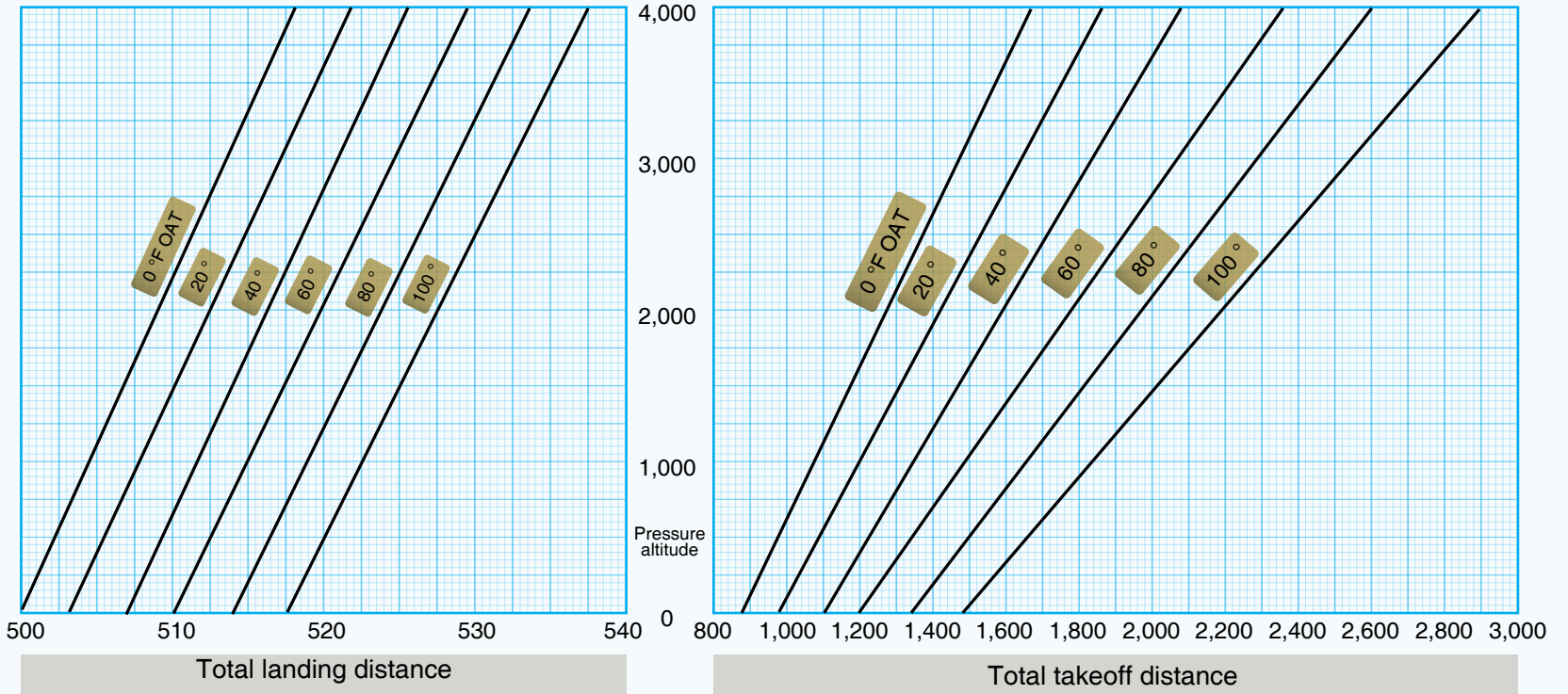
Figure 39. Gyroplane Takeoff and Landing Graphs.
