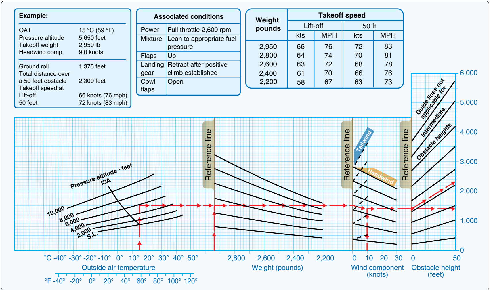
Figure 40. Airplane Takeoff Distance Graph.
