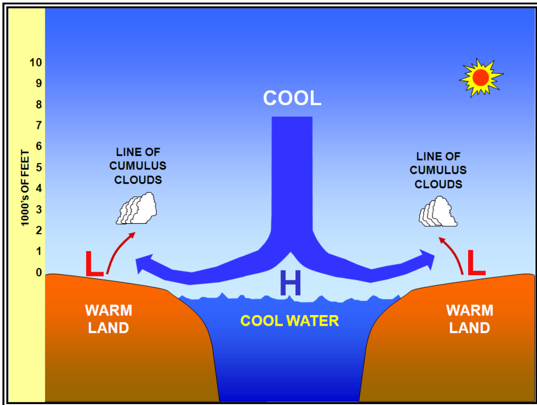
Figure 10-17. Lake Breeze
