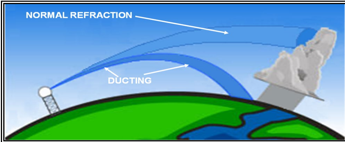
Figure 15-11. Ducting
