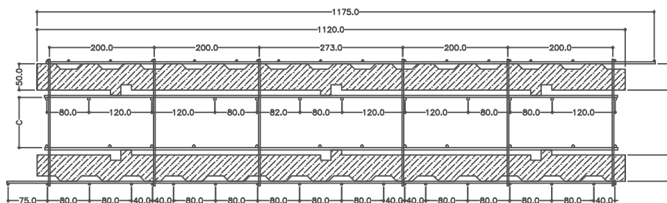
DOUBLE PANEL – Rectangular Profile
