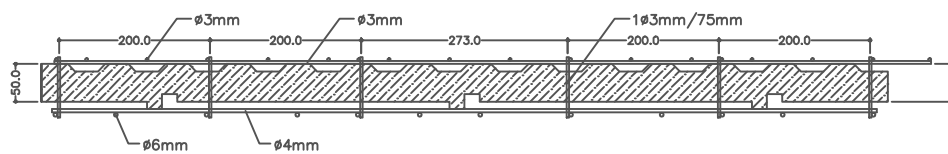
SINGLE PANEL for DOUBLE PANEL – Rectangular Profile
