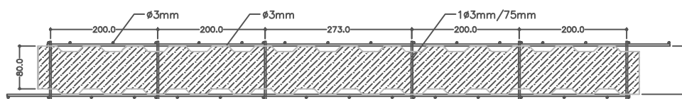
EXTERNAL MESH PANEL SIMPLE Ø3mm
