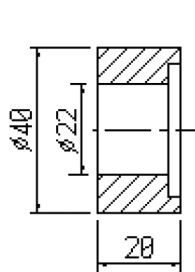
S5/033R roller
