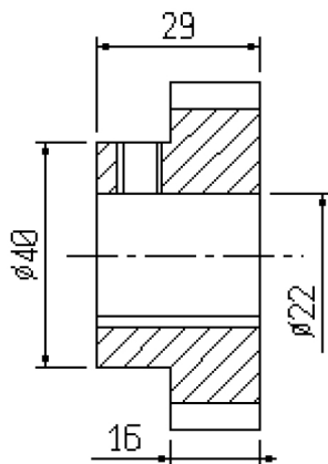
S5/058 Z23 gear SD63d1069
