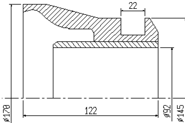
S5/001 sleeve SD50c376
