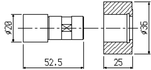
S5/031P (523) pin
