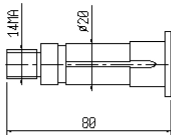
S5/033P pin VD63d851
