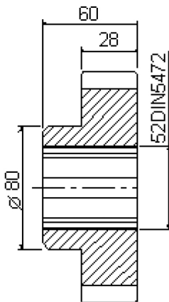
S5/063 Z46 gear SD50d685a
