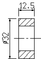
S5/036R roller
