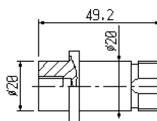
S7/030P (612) pin
