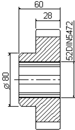
S5/061 Z39 gear SD50d689a
