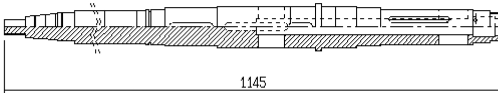
S5/053 clutch-shaft SD50d657d
