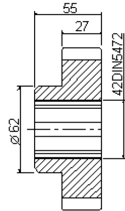
S5/059 Z40 gear SD50d688b
