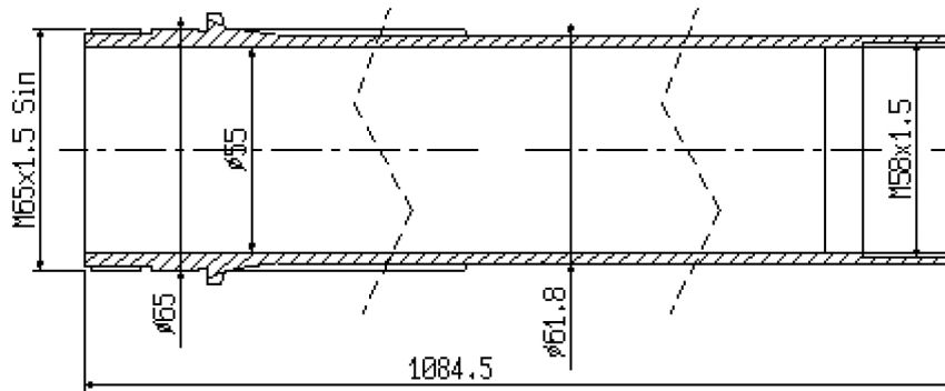
S5/012 feed tube
