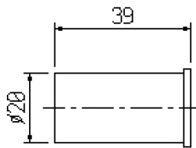
S5/036P pin
