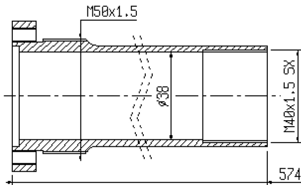
S3/010 collet tube 341
