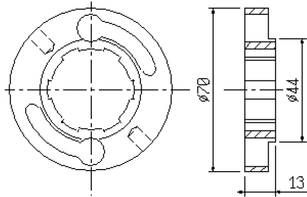
S3/013 Bronze bush 382
