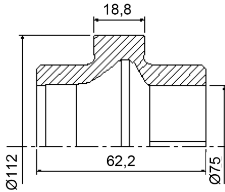
S3/001 sleeve SE25d376
