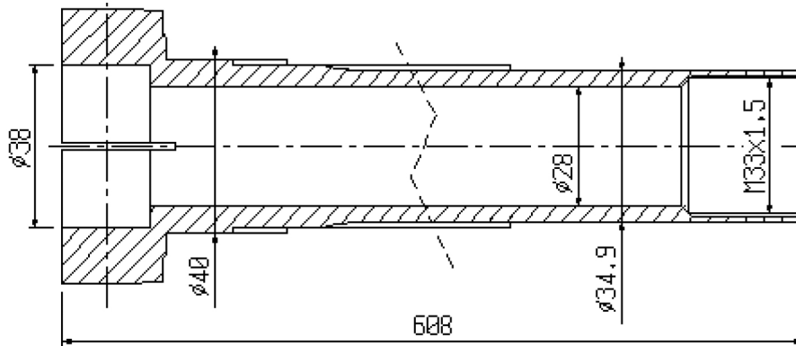
S3/012 feed tube 342
