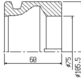
S3/002 sleeve SE25d376b
