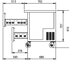
DRAWER MODEL
