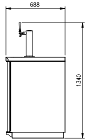
SIDE PLAN
