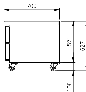
SIDE PLAN
