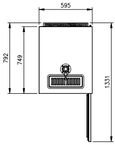
SIDE PLAN
