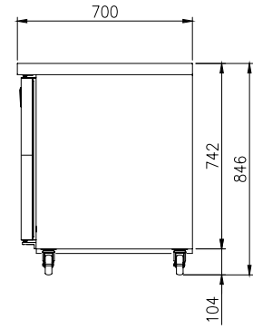
SIDE PLAN
