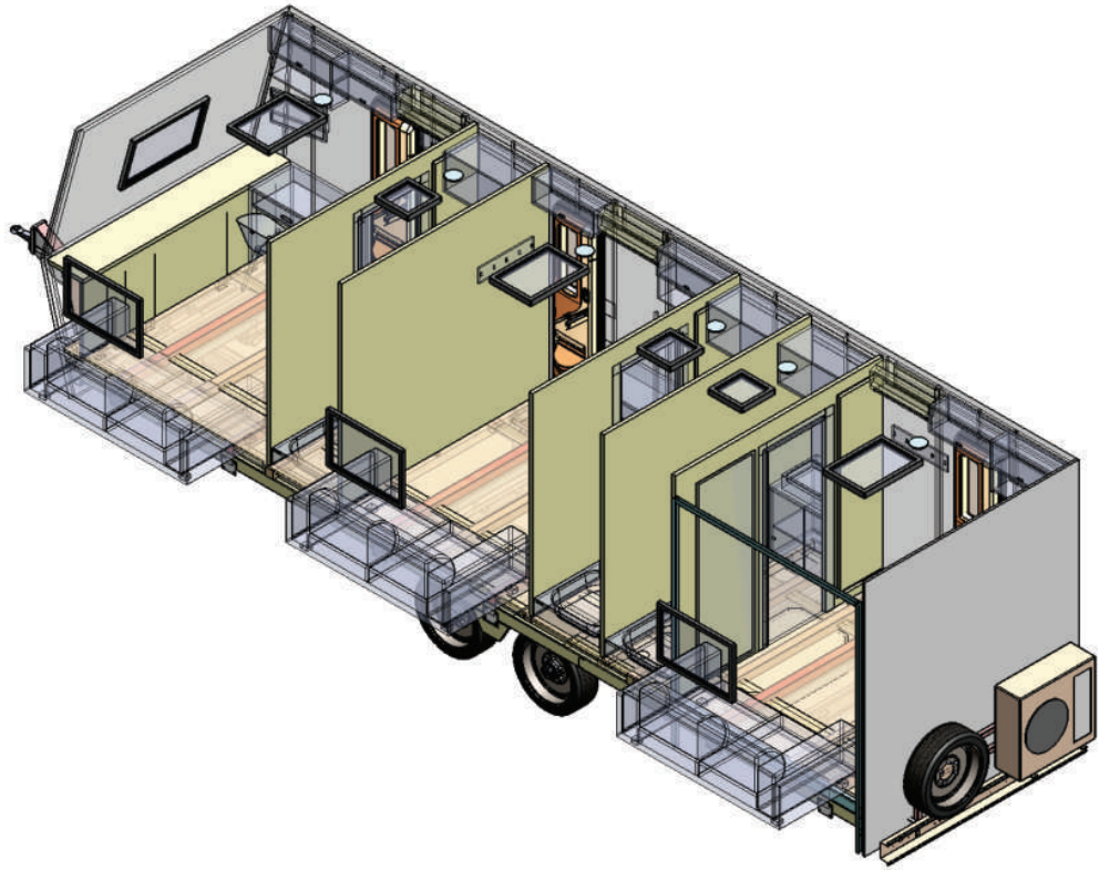
THREE WAY MODEL - TYPE 2016 - 3D VIEW - 03
