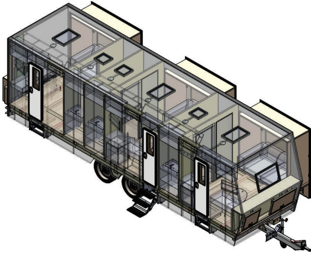
THREE WAY MODEL - TYPE 2016 - 3D VIEW - 01
