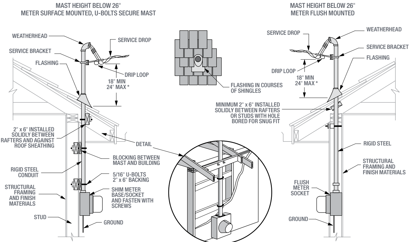
Figure 20 Unguyed service masts
