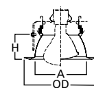
Dimensions** A: 5-3/8" [137mm] H: 2-5/8" [65mm] OD: 7-3/4" [197mm]
