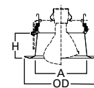
Dimensions** A: 5-3/8" [137mm] H: 2-5/8" [68mm] OD: 7-3/4" [197mm]
