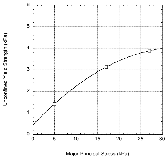
Figure 5.41a. Cohesive strength.
