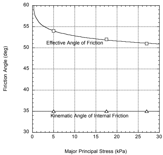
Figure 5.41b. Internal friction.
