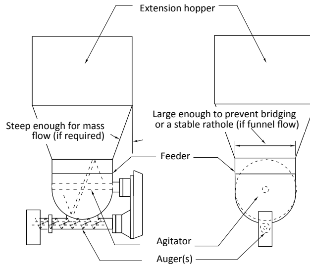
Figure 6.5. Low-throughput screw feeder.
