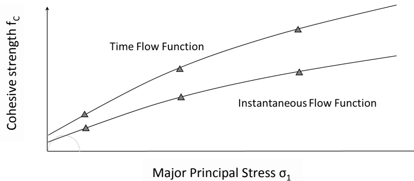
Figure 4.11. Instantaneous and time flow functions.
