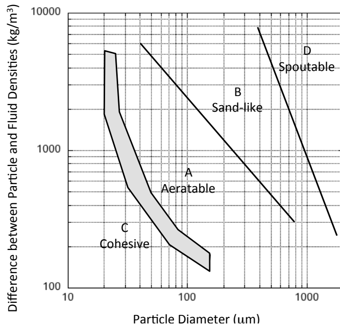
Figure 6.14. Geldart powder classification chart.
