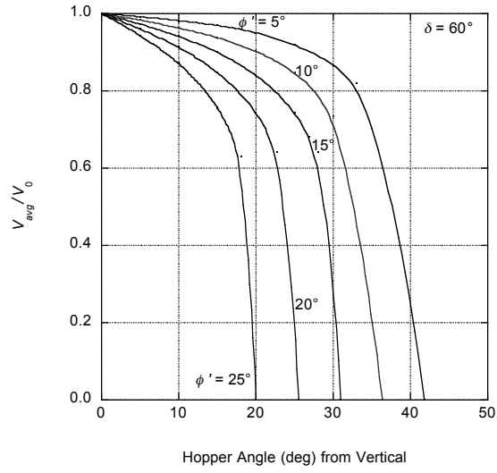
Figure 8.17 Average-centerline velocity ratio, \delta = 60^\circ , axisymmetric flow.
