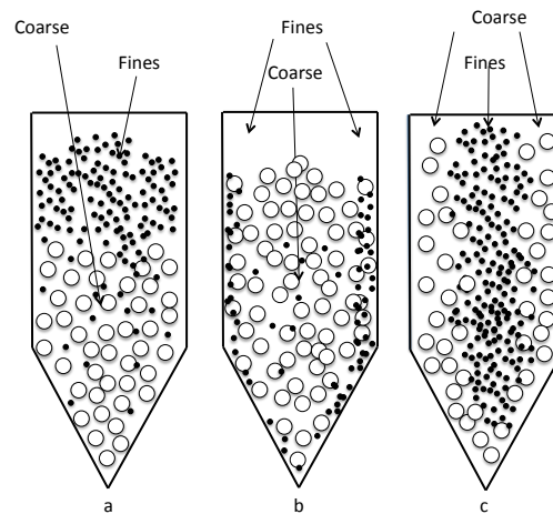
Figure 8.1. Segregation by fluidization (left), dusting (center), and sifting (right).
