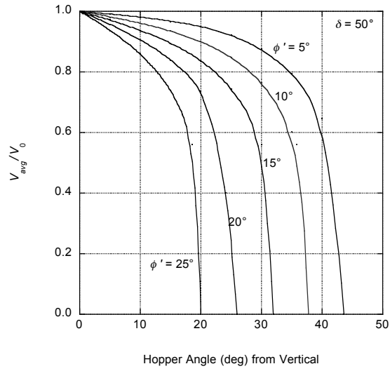
Figure 8.16 Average-centerline velocity ratio, \delta = 50^\circ , axisymmetric flow.
