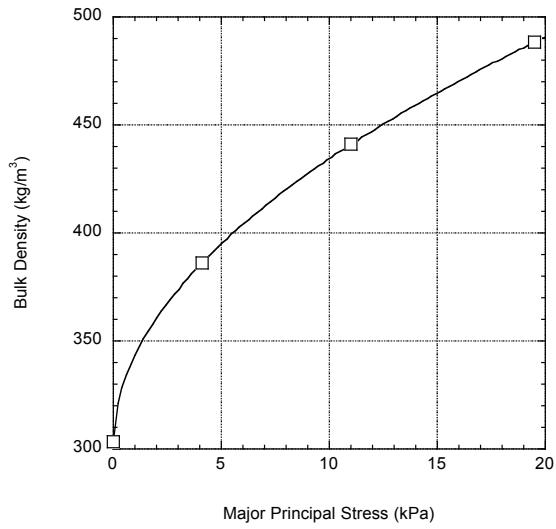
Figure 5.37c. Compressibility.
