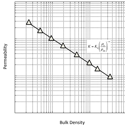
Figure 4.21. Bulk density – permeability relationship.
