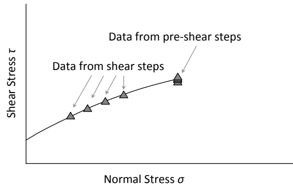
Figure 4.6. Yield locus.
