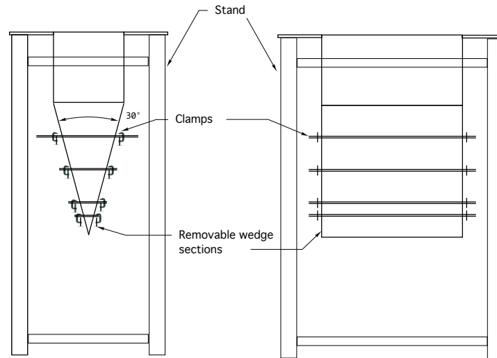
Figure 4.22. Hopper test apparatus.
