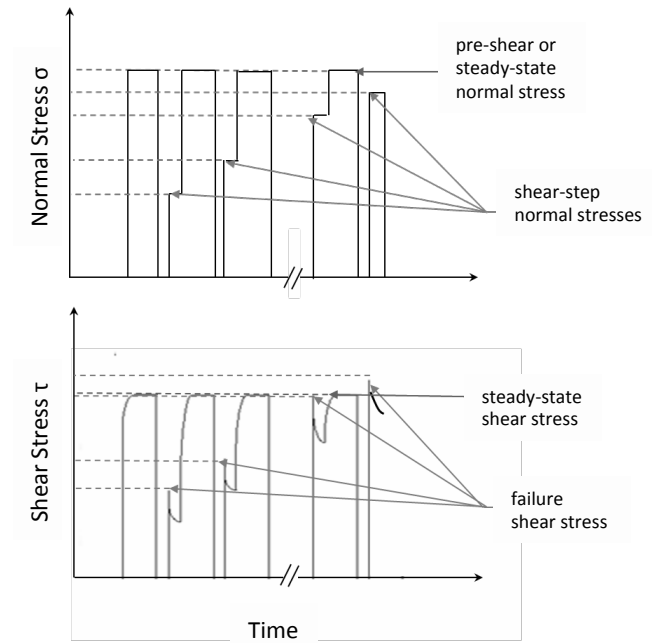
Figure 4.5. Pre-shear and shear steps.
