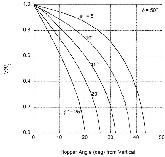
Figure 8.8. Wall-centerline velocity ratio, \delta = 50^\circ , axisymmetric flow.
