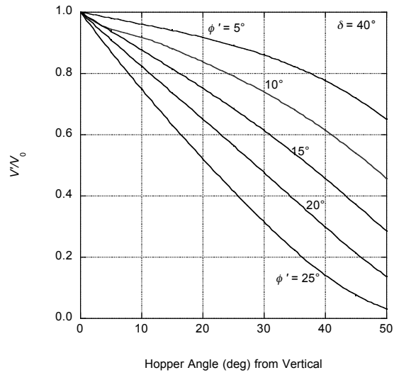
Figure 8.11. Wall-centerline velocity ratio, \delta = 40^\circ , planar flow.
