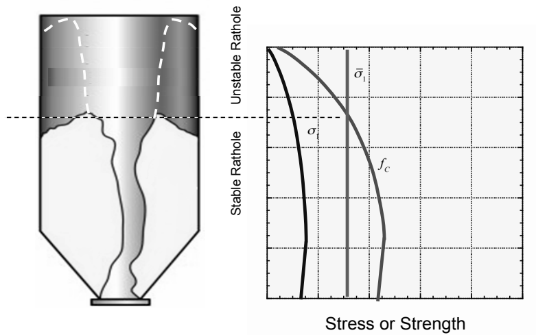
Figure 5.25. Formation of a stable rathole in a funnel flow hopper.
