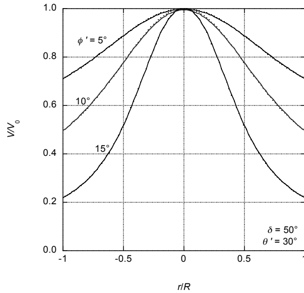
Figure 8.5. Velocity profiles for \delta = 50^\circ , \theta = 30^\circ , axisymmetric flow.
