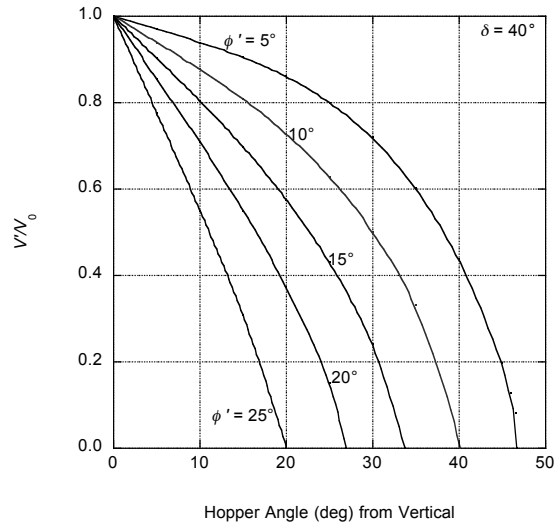
Figure 8.7. Wall-centerline velocity ratio, \delta = 40^\circ , axisymmetric flow.
