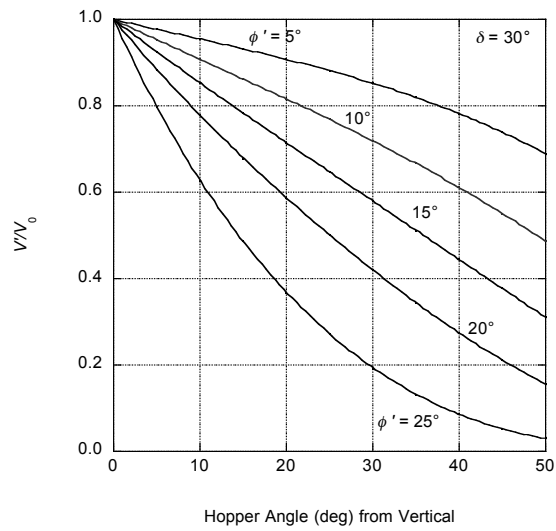
Figure 8.10. Wall-centerline velocity ratio, \delta = 30^\circ , planar flow.
