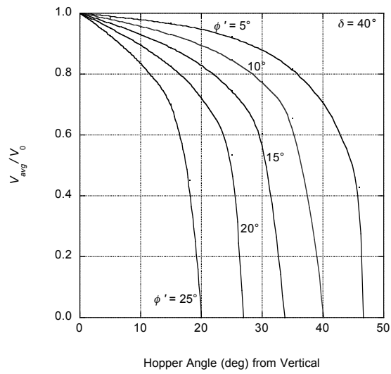
Figure 8.15. Average-centerline velocity ratio, \delta = 40^\circ , axisymmetric flow.
