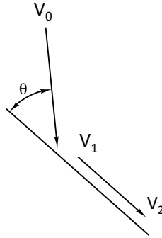
Figure 8.24. Velocity after impact and sliding.
