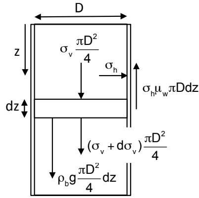
Figure 3.2. Stresses on element of bulk solid inside cylinder.
