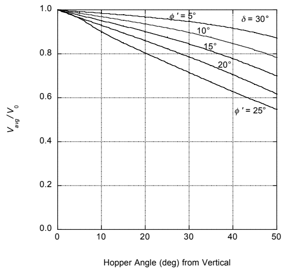
Figure 8.18. Average-centerline velocity ratio, \delta = 30^\circ , planar flow.
