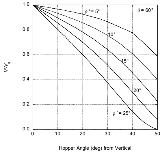
Figure 8.13. Wall-centerline velocity ratio, \delta = 60^\circ , planar flow.
