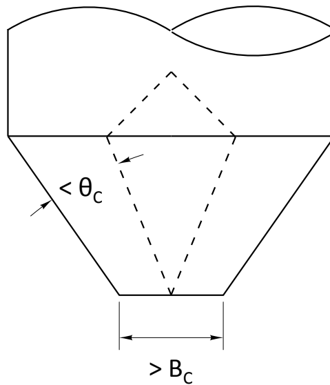
Figure 5.30. Lyn Bates' bullet insert.
