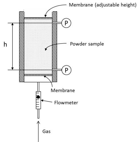
Figure 4.19. Permeability tester.
