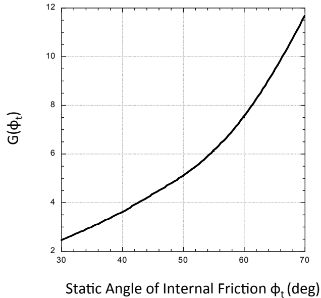
Figure 5.24. Function G(\phi_t) .
