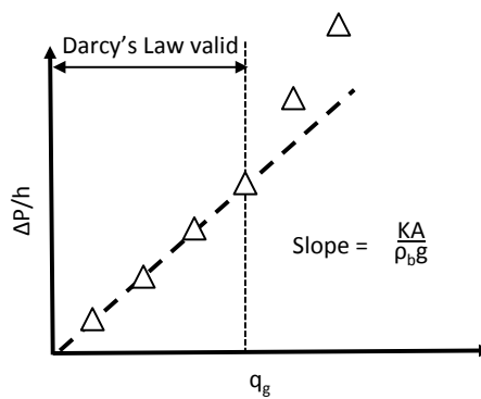
Figure 4.20. Determination of K from permeability test results.
