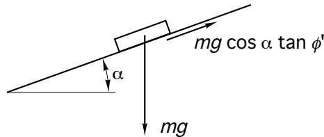
Figure 7.2. Element of bulk solid sliding on a straight chute.
