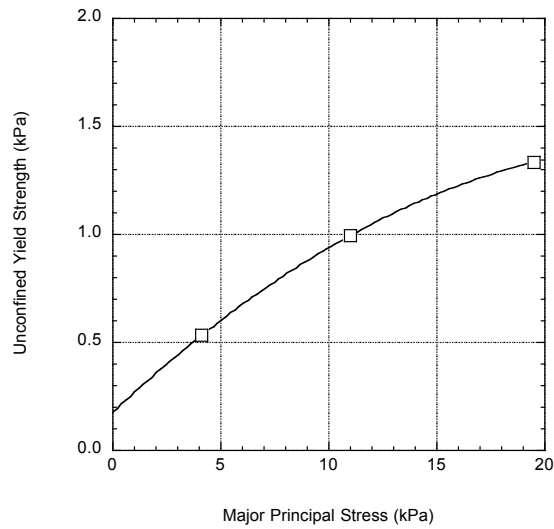
Figure 5.37a. Flow function.
