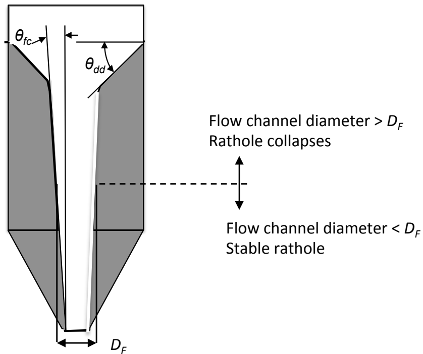
Figure 5.34. Flow channel and drawdown angles.
