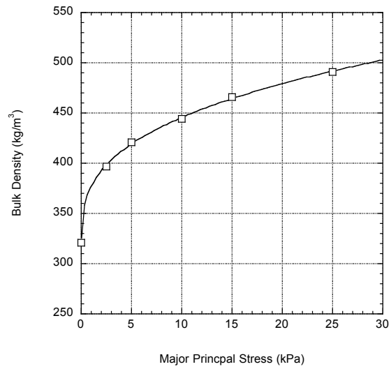
Figure 5.39c. Compressibility.
