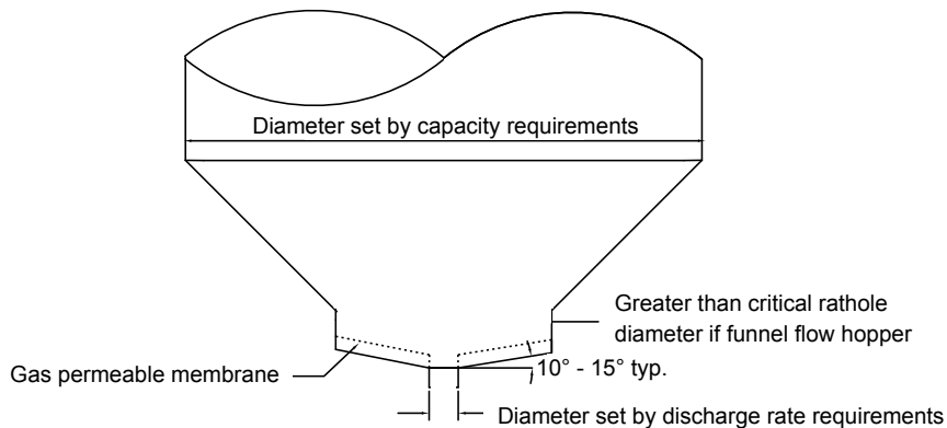
Figure 6.13. Fluidized discharger.
