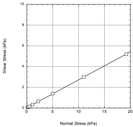
Figure 5.37d. Wall yield locus.
