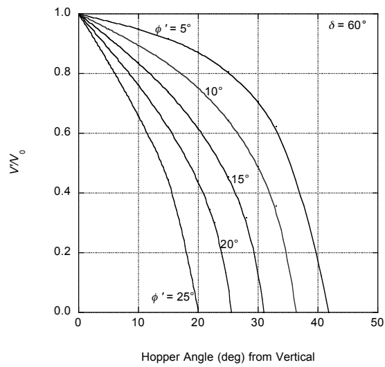
Figure 8.9. Wall-centerline velocity ratio, \delta = 60^\circ , axisymmetric flow.
