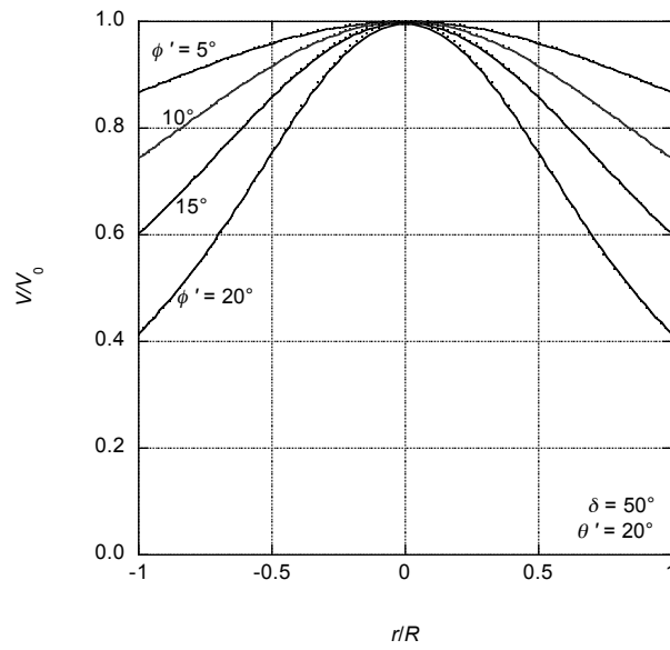
Figure 8.4. Velocity profiles for \delta = 50^\circ , \theta = 20^\circ , axisymmetric flow.
