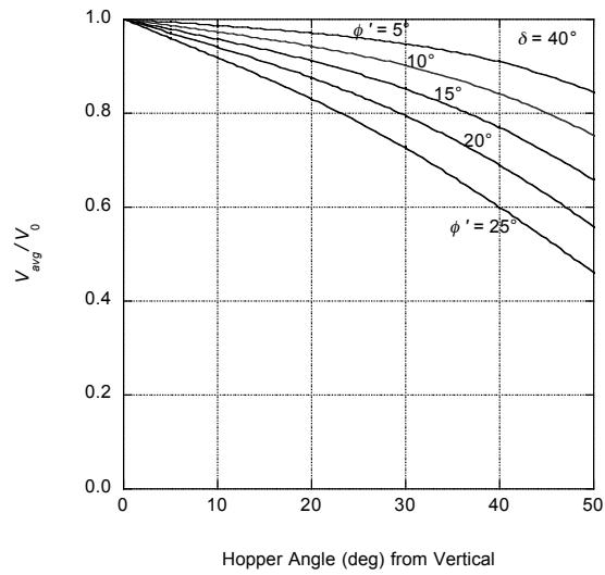
Figure 8.19. Average-centerline velocity ratio, \delta = 40^\circ , planar flow.
