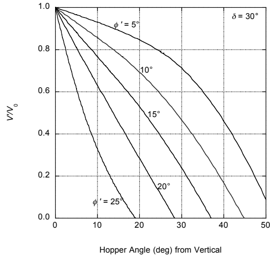
Figure 8.6. Wall-centerline velocity ratio, \delta = 30^\circ , axisymmetric flow.
