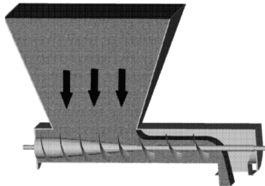
Figure 6.4. Mass flow screw feeder.
