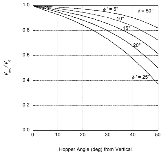
Figure 8.20. Average-centerline velocity ratio, \delta = 50^\circ , planar flow.
