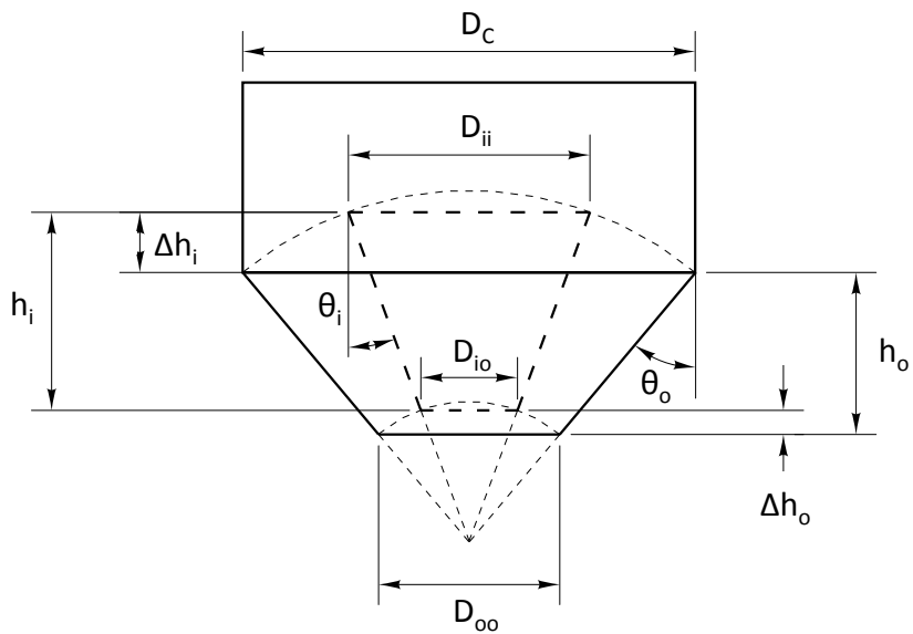
Figure 5.28. Insert geometry.
