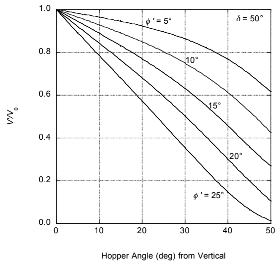
Figure 8.12. Wall-centerline velocity ratio, \delta = 50^\circ , planar flow.
