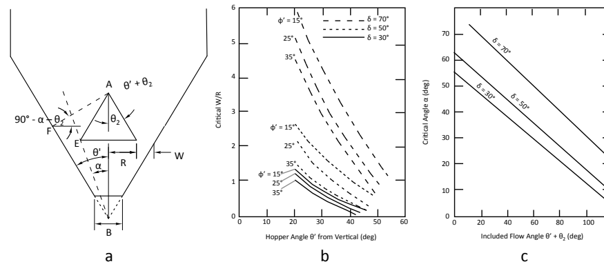
Figure 5.31. Inverted-cone insert.
