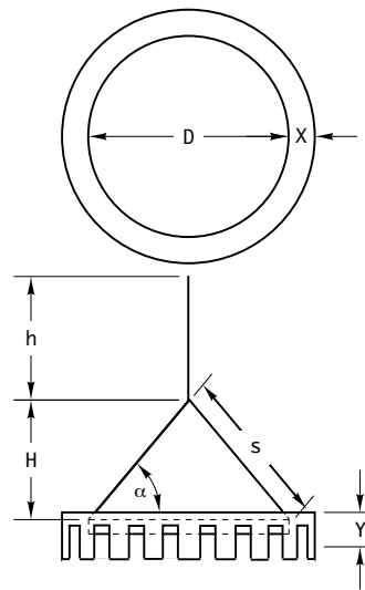
Figure 8.23. Dispersion cone and ring dimensions.
