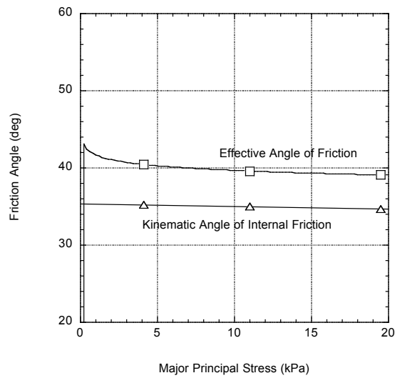
Figure 5.37b. Internal friction.
