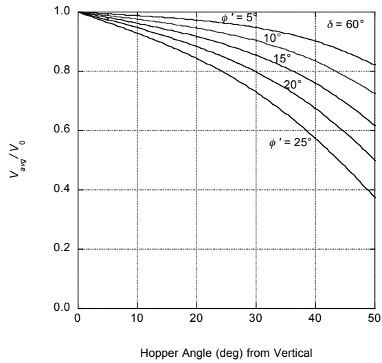
Figure 8.21. Average-centerline velocity ratio, \delta = 60^\circ , planar flow.
