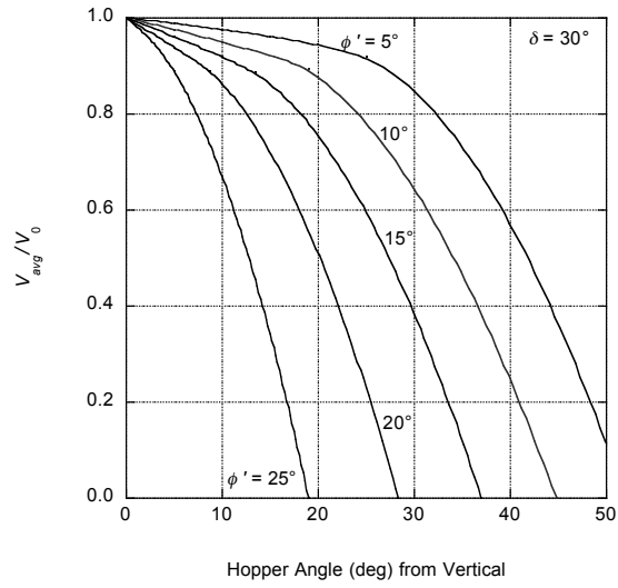
Figure 8.14. Average-centerline velocity ratio, \delta = 30^\circ , axisymmetric flow.
