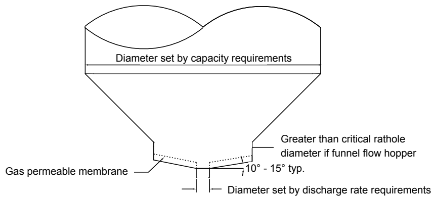
Figure 6.13. Fluidized discharger.
