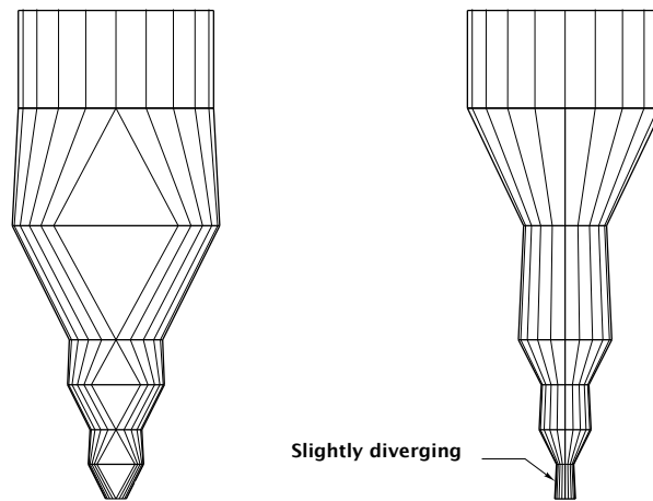
Figure 5.32. Diamondback hopper.
