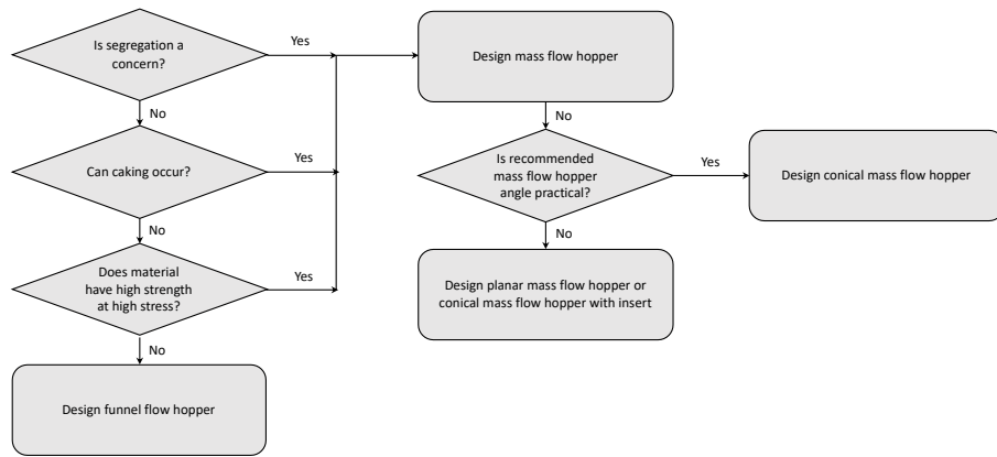
Figure 5.37. Bin design procedure.
