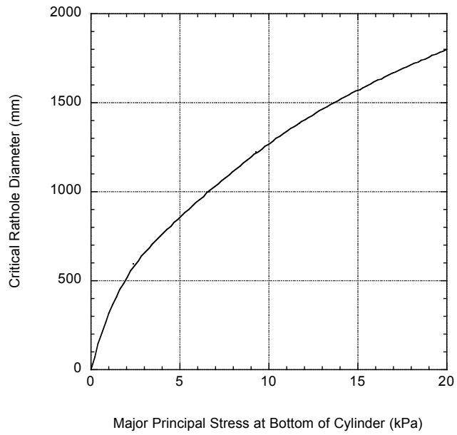
Figure 5.40. Critical rathole diameter.
