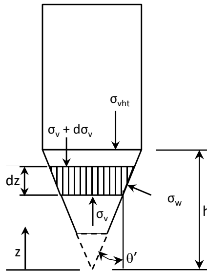
Figure 3.7. Forces acting on a differential slice of bulk material in a hopper.
