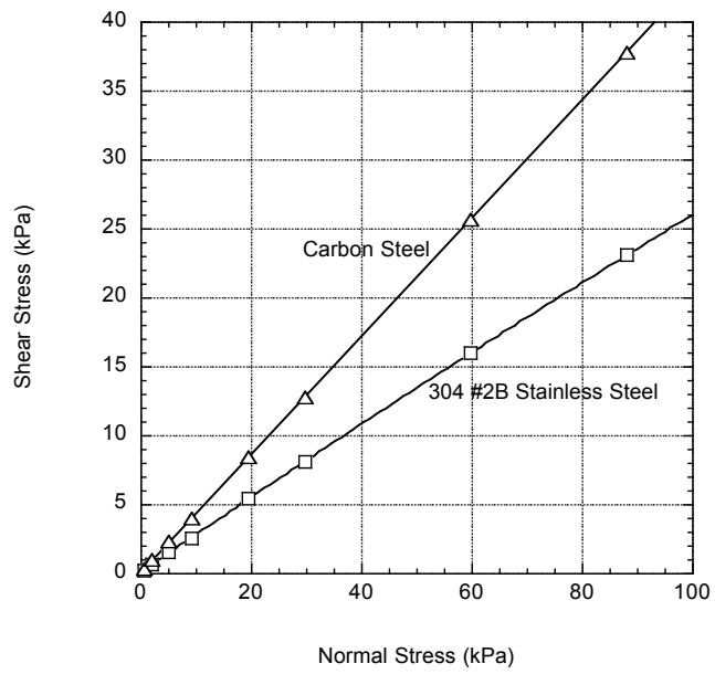
Figure 5.39d. Wall friction.
