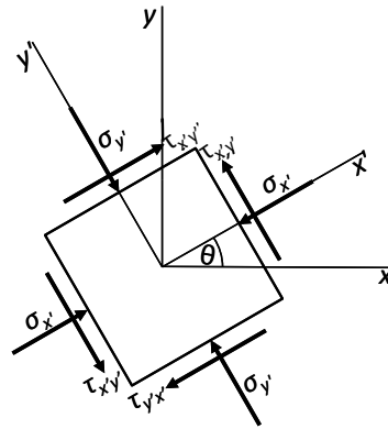
Figure 2.5. Stresses on a rotated element.
