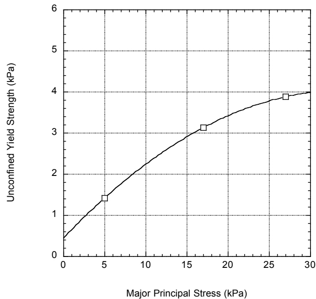
Figure 5.39a. Cohesive strength.
