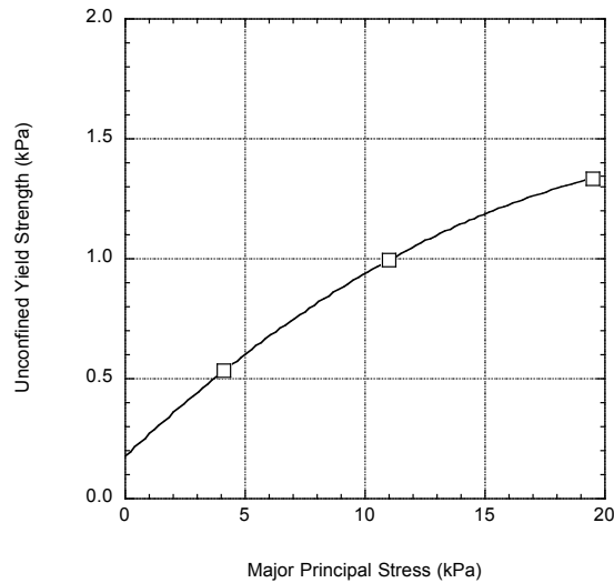
Figure 5.38a. Flow function.
