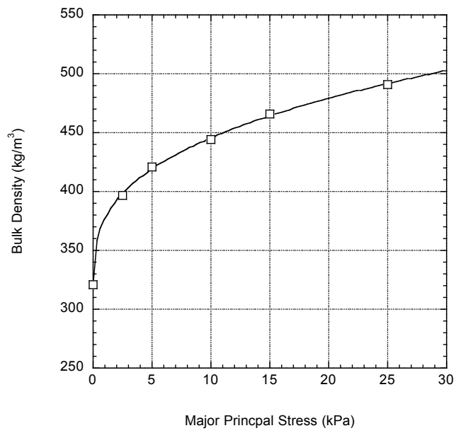
Figure 5.39c. Compressibility.
