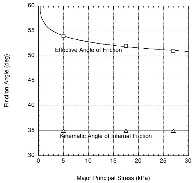
Figure 5.39b. Internal friction.
