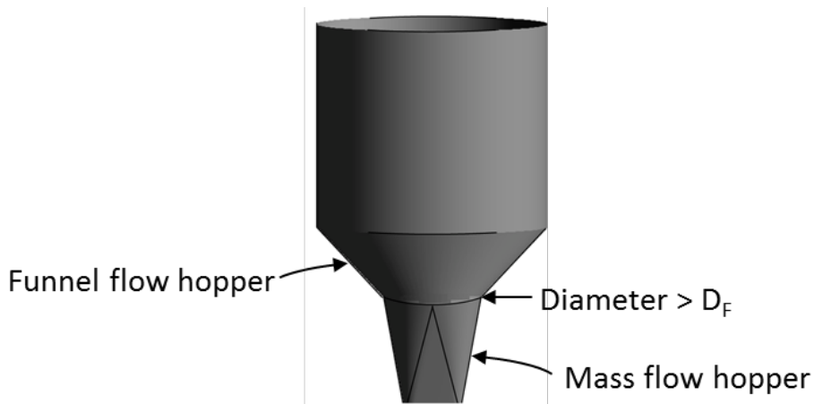
Figure 5.26. Expanded flow hopper.
