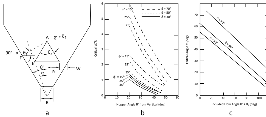
Figure 5.31. Inverted-cone insert.
