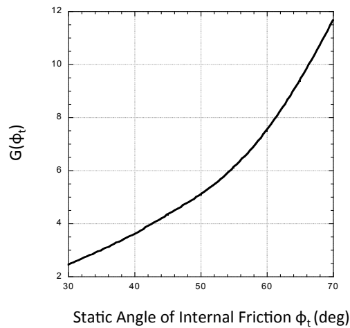
Figure 5.24. Function G(\phi_i) .
