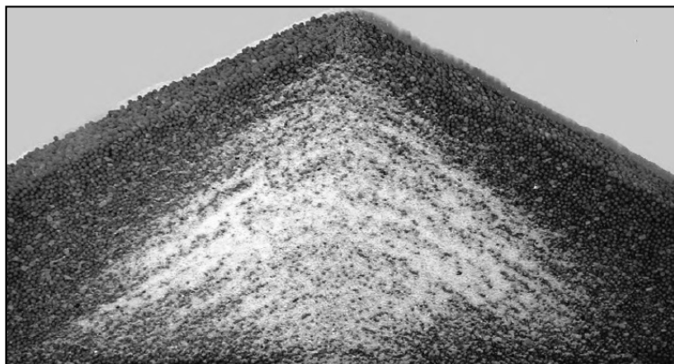
Figure 7.2. Sifting segregation after formation of a pile.
