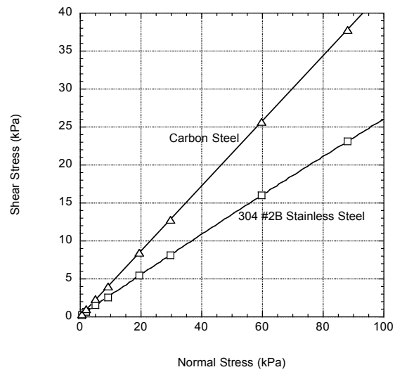
Figure 5.39d. Wall friction.
