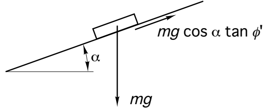
Figure 7.28. Element of bulk solid sliding on a straight chute.
