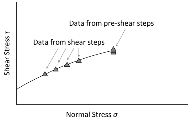
Figure 4.6. Yield locus.
