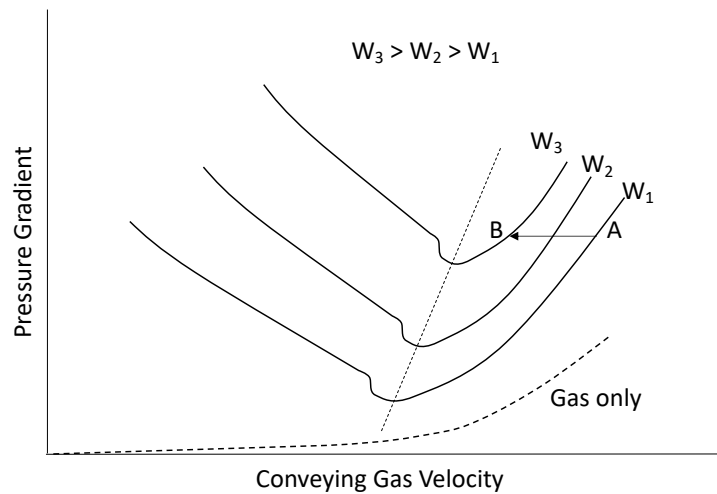
Figure 7.37. Optimization of conveying system.
