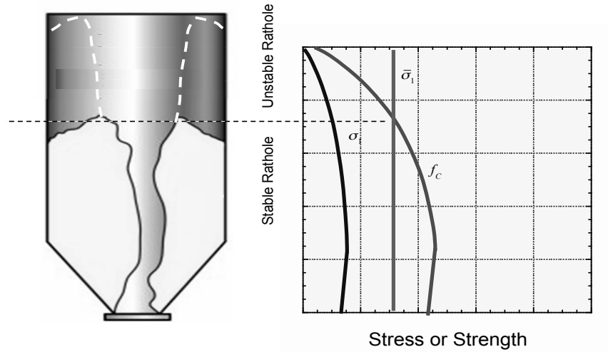
Figure 5.25. Formation of a stable rathole in a funnel flow hopper.
