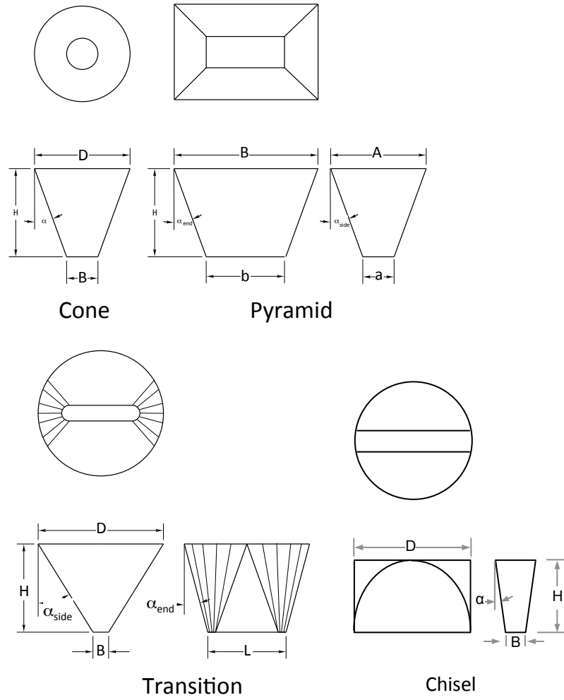
Figure 5.35. Conical, pyramidal, and transition hopper nomenclature.
