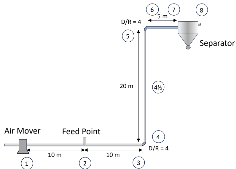
Figure 7.39. Proposed dilute-phase conveying system.
