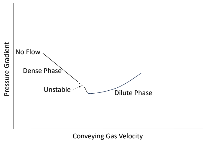
Figure 7.36. State diagram.
