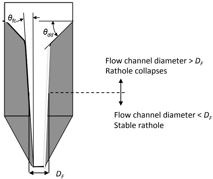
Figure 5.34. Flow channel and drawdown angles.
