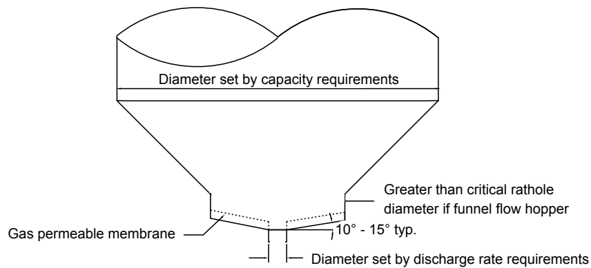
Figure 6.13. Fluidized discharger.
