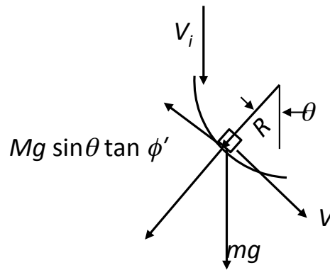
Figure 7.42. Element of bulk solid sliding on a curved chute.
