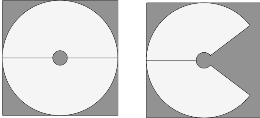
Figure 5.3. Fabrication of 30° (left) and 20° (right) hoppers.
