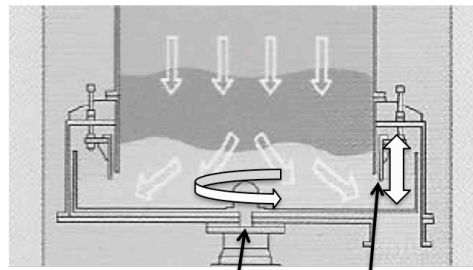
Figure 6.11. LCI Circle feeder.
