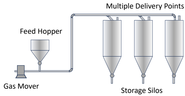
Figure 7.34. Pressure system.
