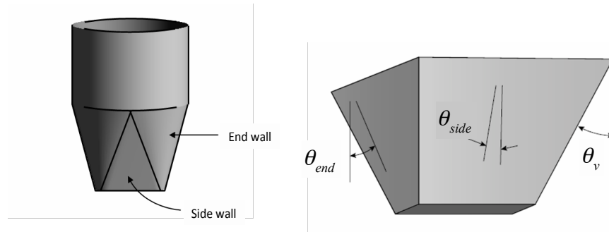
Figure 5.5. Side and end walls of transition hopper (left) and side, end, and valley angles of pyramidal hoppers (right).
