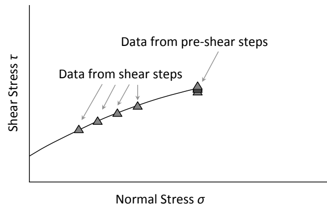
Figure 4.6. Yield locus.
