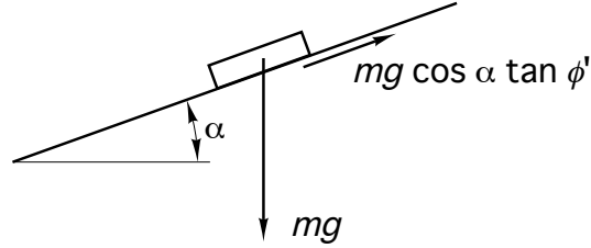
Figure 7.41. Element of bulk solid sliding on a straight chute.
