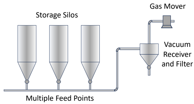
Figure 7.35. Vacuum system.
