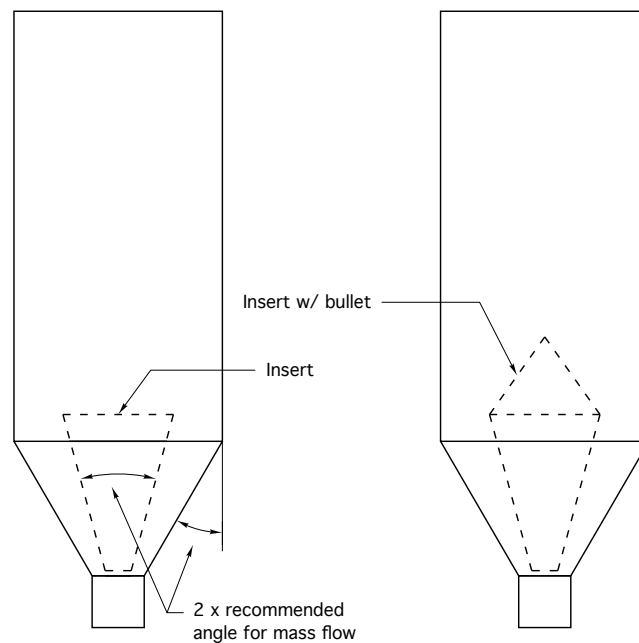
Figure 5.27. Inserts; cone-in-cone, left, and bullet, right.
