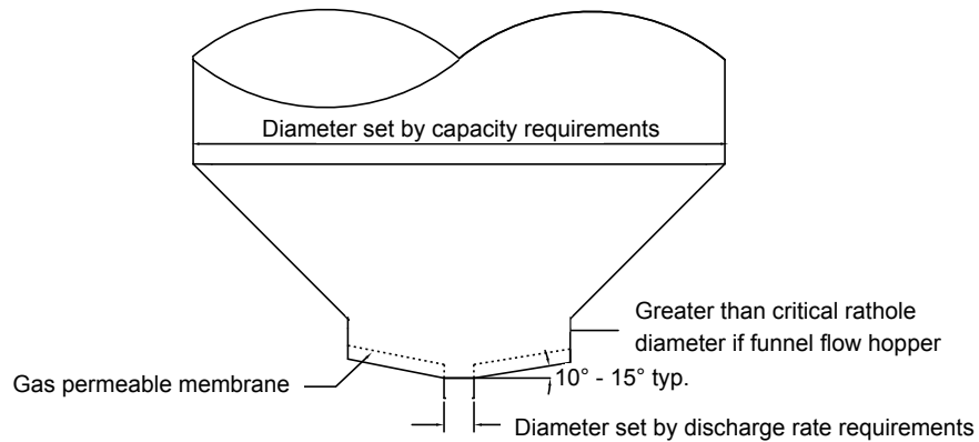
Figure 6.13. Fluidized discharger.
