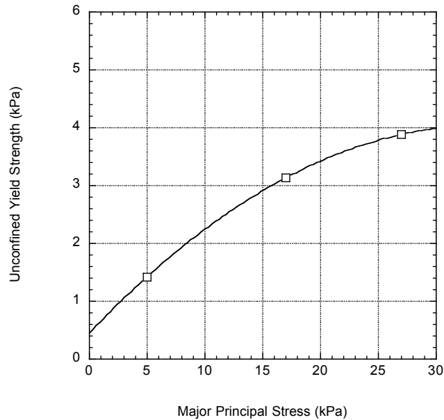
Figure 5.41a. Cohesive strength.
