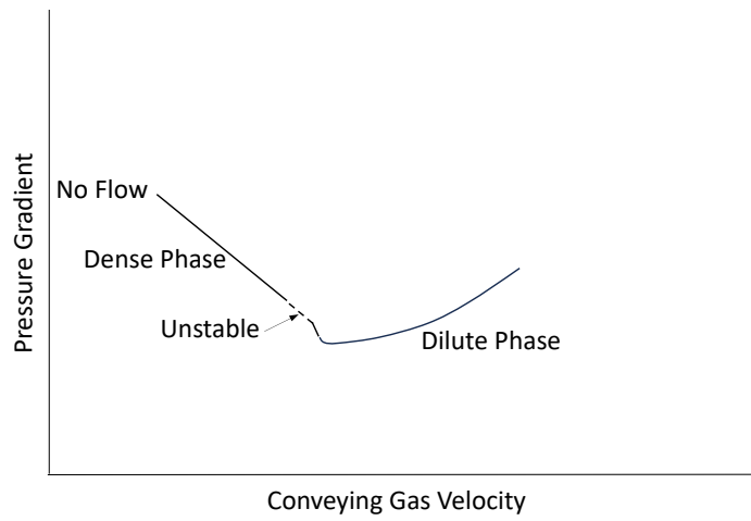
Figure 7.38. State diagram.
