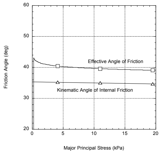
Figure 5.40b. Internal friction.
