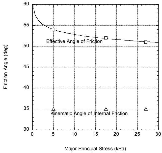
Figure 5.41b. Internal friction.
