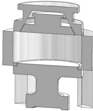
Figure 4.25. Johanson indicizer.
