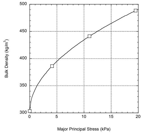
Figure 5.40c. Compressibility.
