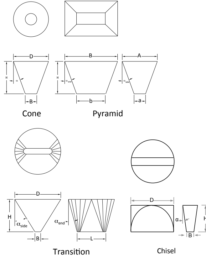
Figure 5.37. Conical, pyramidal, and transition hopper nomenclature.
