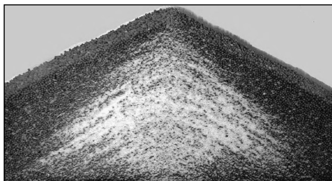
Figure 7.2. Sifting segregation after formation of a pile.
