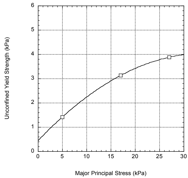
Figure 5.41a. Cohesive strength.
