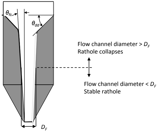
Figure 5.36. Flow channel and drawdown angles.
