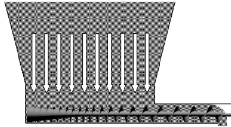
Figure 6.4. Mass flow screw feeder.
