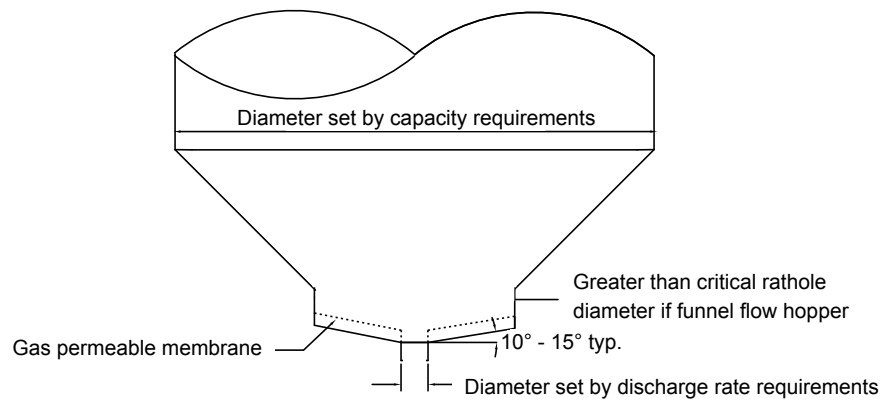
Figure 6.13. Fluidized discharger.
