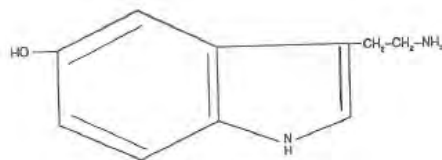
SEROTONIN
