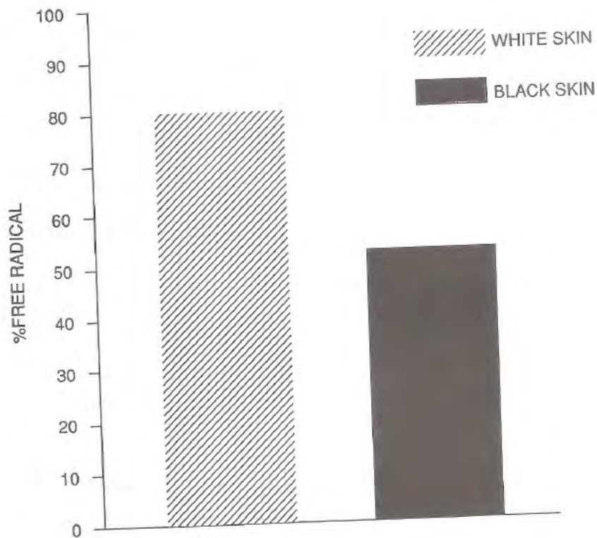
FIGURE 6A FREE RADICAL PRODUCTION IN EDIPERMAL PROTEIN (SKIN) BY ULTRAVIOLET IRRADIATION*
