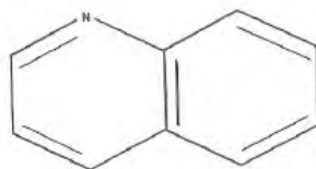
QUINOLINE
