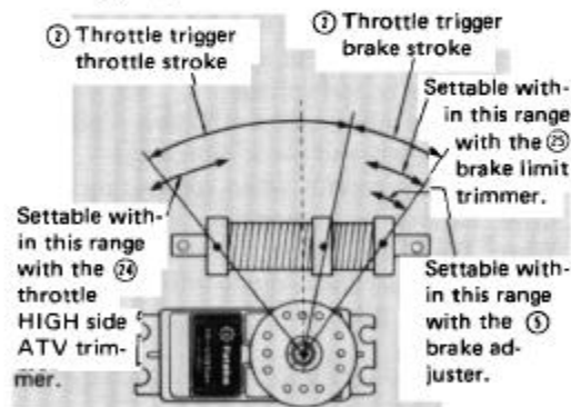
Throttle (engine control servo) Fig. 21
