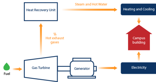
How cogeneration works
