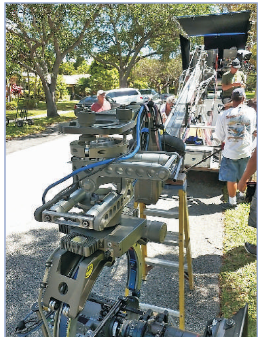
Libra Head with ISO Dampener and GF-6 Crane
