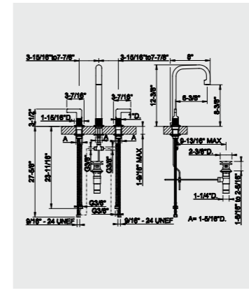
58015 Three-hole basin mixer 58016 Without pop-up
