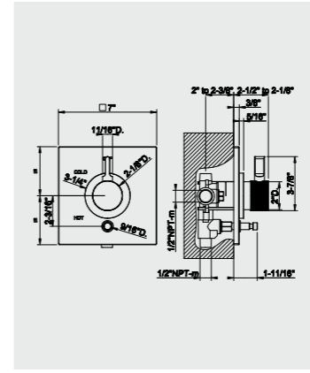
09274_58174 Pressure balance 09272_58173
