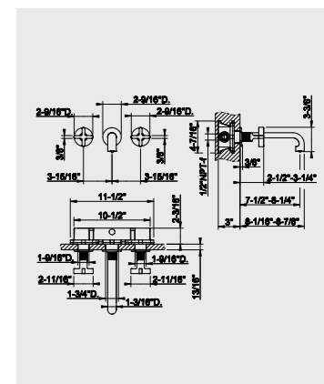
48089_58190 Built-in three-hole basin mixer 48089_58192 without pop-up
