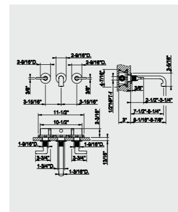
48089_58090 Built-in three-hole basin mixer 48089_58092 without pop-up
