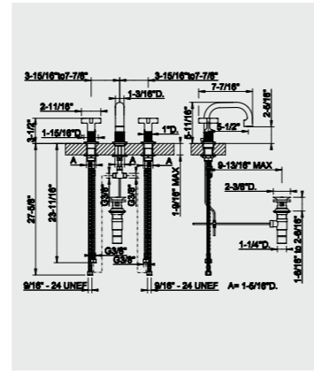
58111 Three-hole basin mixer 58112 Without pop-up
