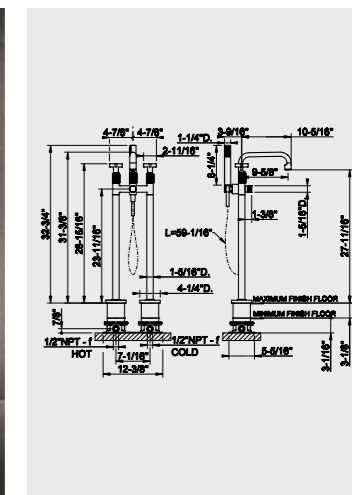
58099_58128 Freestanding external bath mixer
