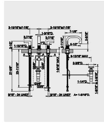
58011 Three-hole basin mixer 58012 Without pop-up
