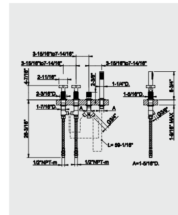
58143 Four-hole bath mixer
