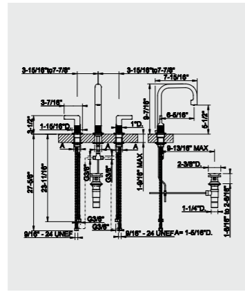
58013 Three-hole basin mixer 58014 Without pop-up
