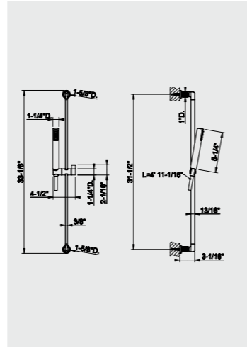
58145 Sliding rail
