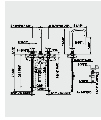
58115 Three-hole basin mixer 58116 Without pop-up
