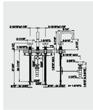
58113 Three-hole basin mixer 58114 Without pop-up
