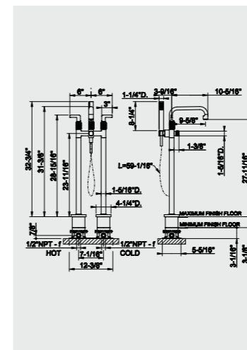
58099_58028 Freestanding external bath mixer
