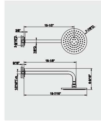
58148 Wall-mounted showerhead
