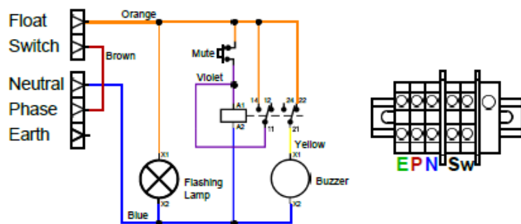
Circuit Diagram
