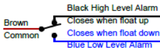
High level alarm, low level alarm float switch wiring
