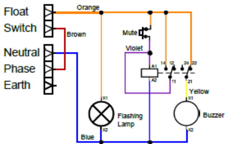
Circuit Diagram
