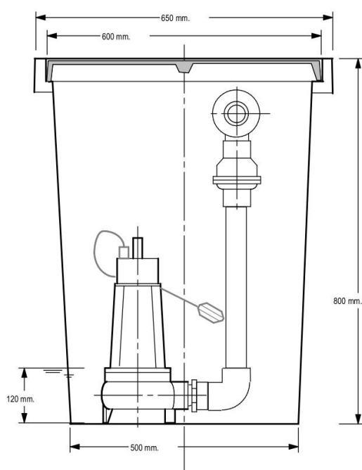
Side Elevation
