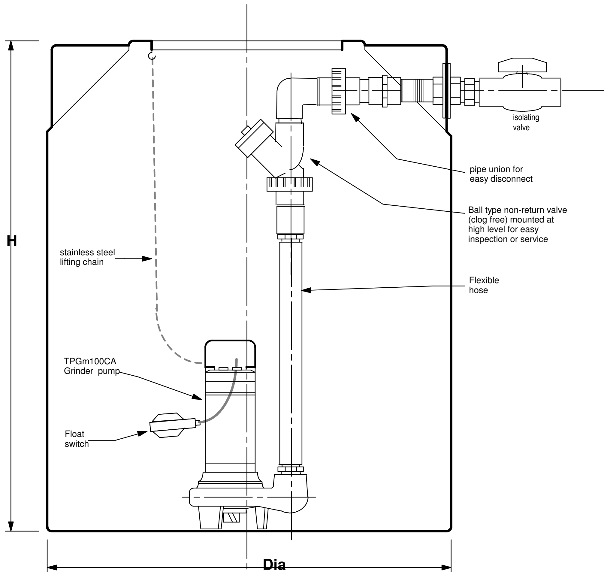
Tank Dimensions (mm)
