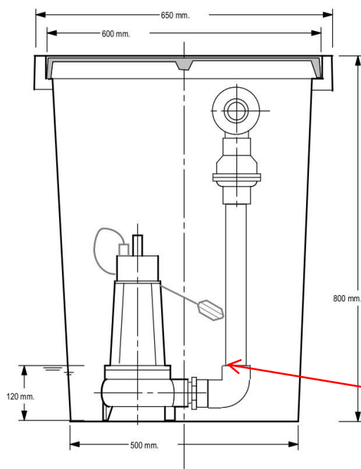
Side Elevation
