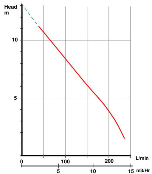
150 SP-6 TPG-100 Pump
