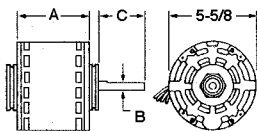
BELLY BAND OR RING MOUNT
