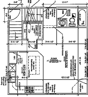
2 Main Level Plan SCALE: 1/4"=1'-0"
