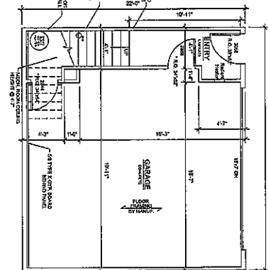
1 Garage Plan SCALE: 1/4"=1'-0"
