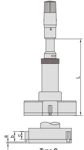
Type C 2-12", carbide points
