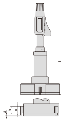
Type C 2-12", carbide points
