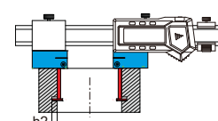
Measuring internal groove diameter with spherical measuring face (depth h2 \leq .295" )
