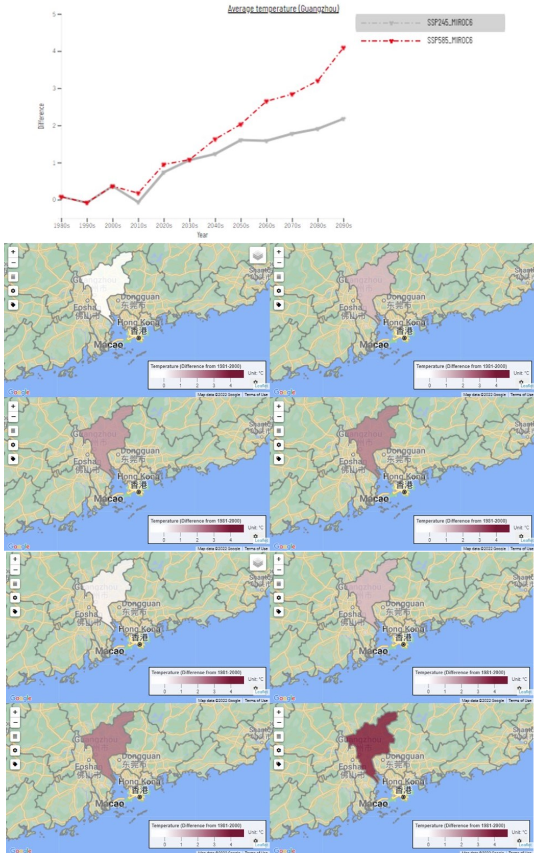
Figure 5.20: Temperature increase in Guangzhou under medium (grey) and high (red) emission scenario till 2080s (top); Spatial results for medium scenario for 2010s, 2030s, 2050s, 2080s (middle); Spatial results for high scenario for 2020s, 2030s, 2050s, 2080s (bottom)
