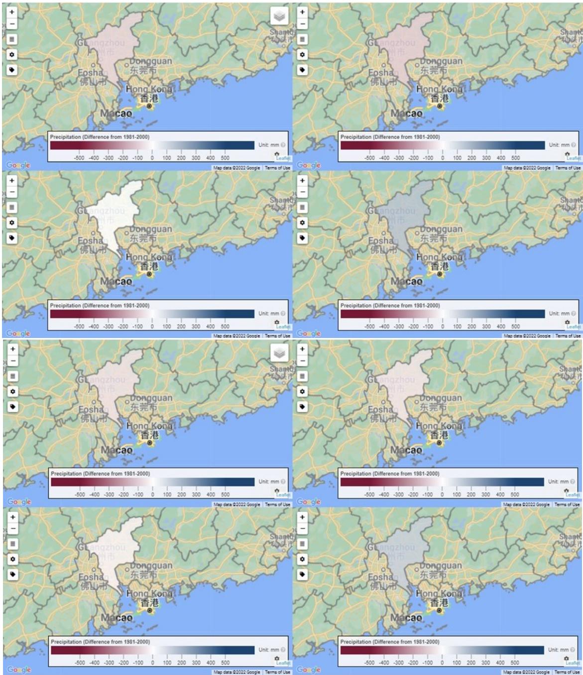
Figure 5.21: Precipitation variation in Guangzhou under medium (grey) and high (red) emission scenario till 2080s (top); Spatial results for medium scenario for 2010s, 2030s, 2050s, 2080s (middle); Spatial results for high scenario for 2020s, 2030s, 2050s, 2080s (bottom)
