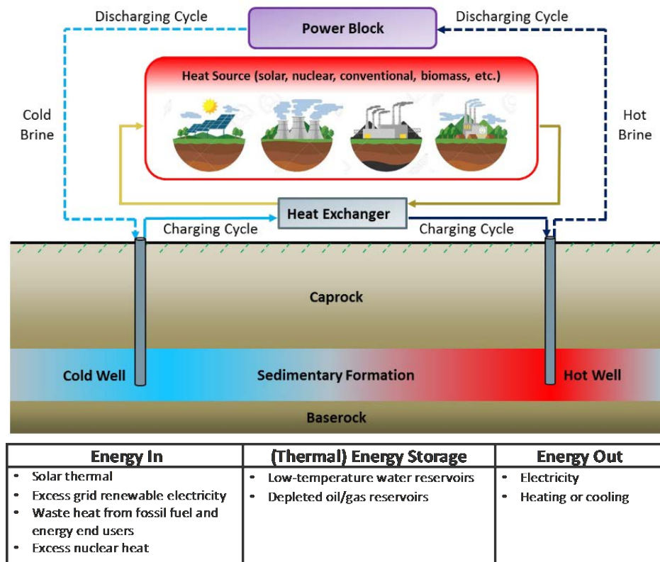
Figure 1: Illustration of GeTES technologies and processes.
