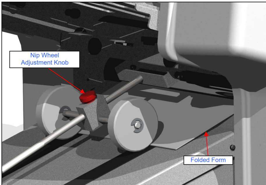
Figure 10: Nip Wheel Adjustment
