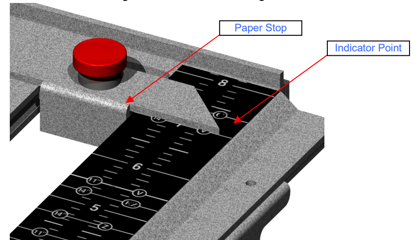
Figure 9: Paper Stop Alignment
