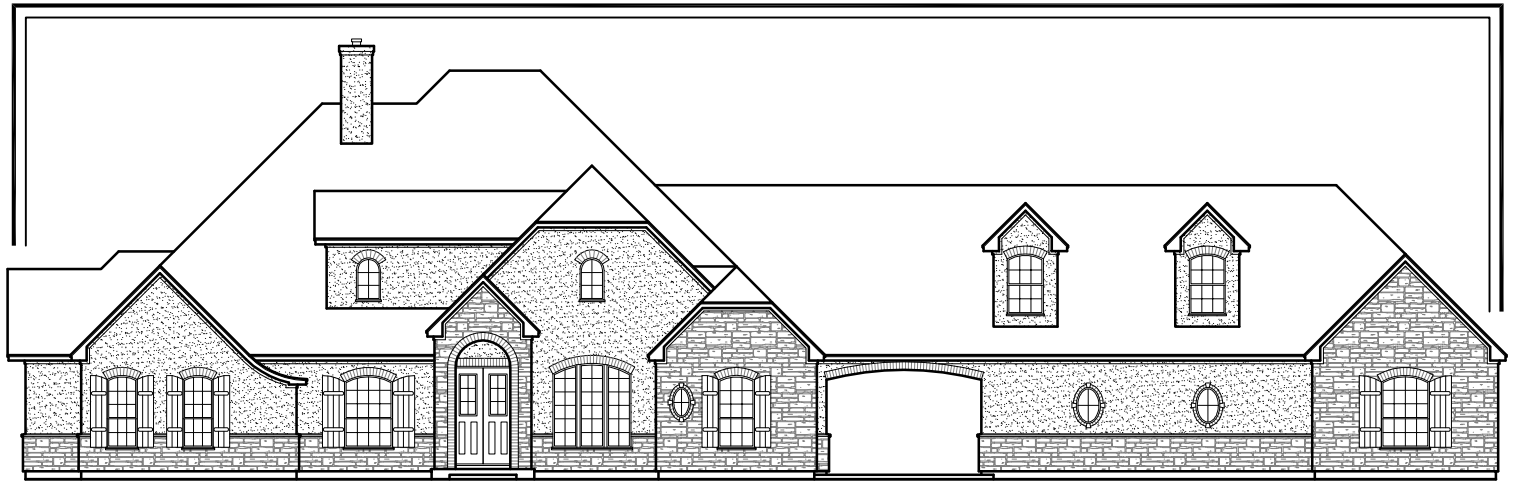
③ Front Elevation
