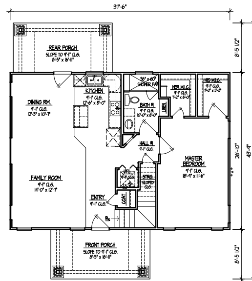
Architectural 1st Floor Plan ①
