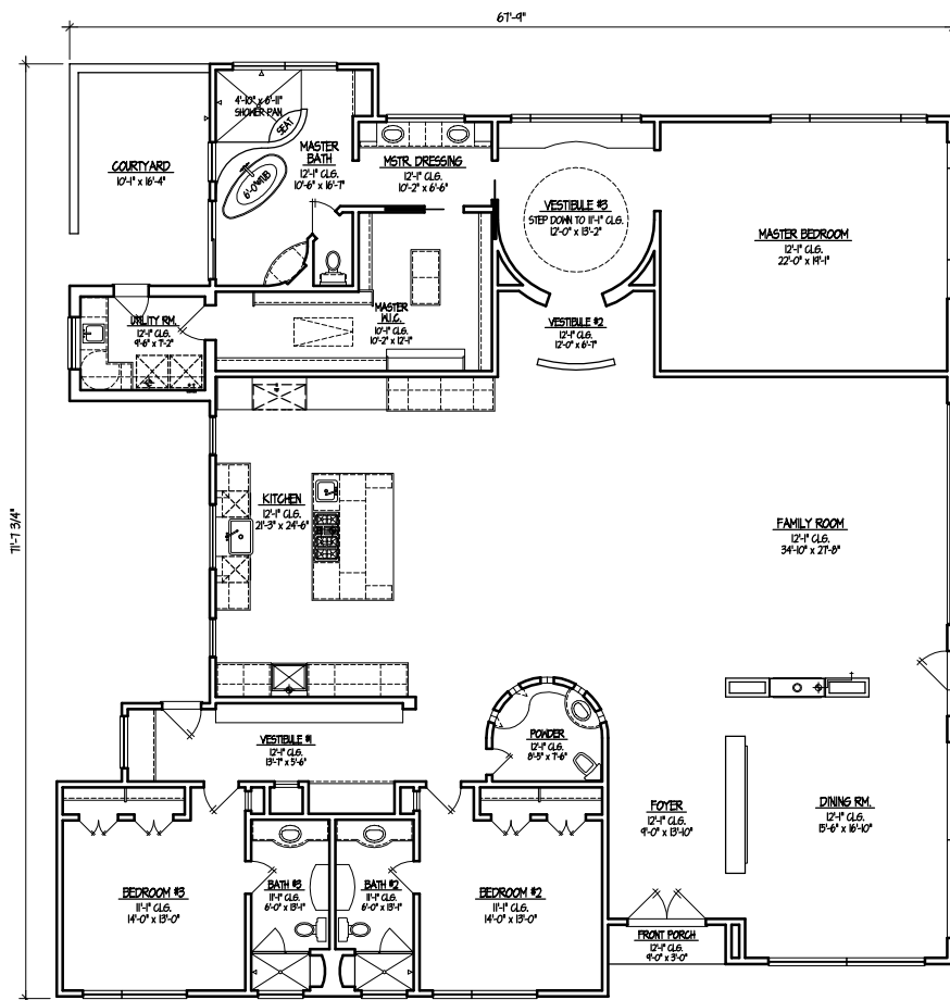
Architectural Floor Plan
