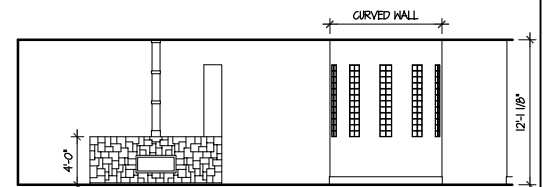
Int. Elev. at Family Room
