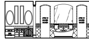
Int. Elev. at Master Bath 4
